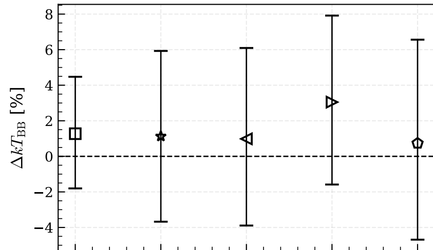
GBM-only vs Joint
