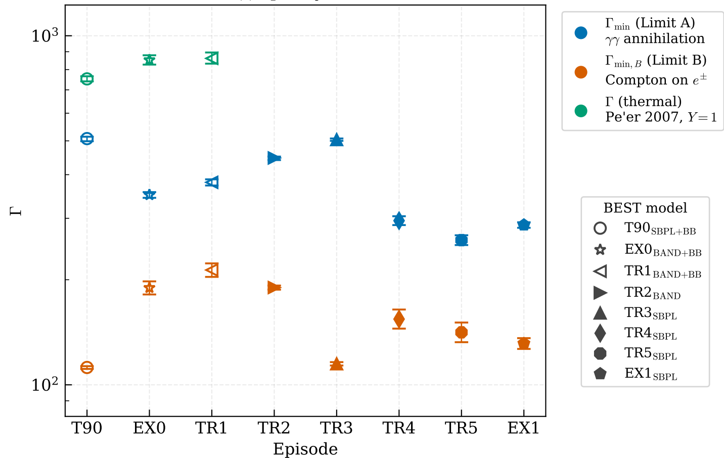
GRB080916C: \gamma -opacity limits vs. Thermal \Gamma
