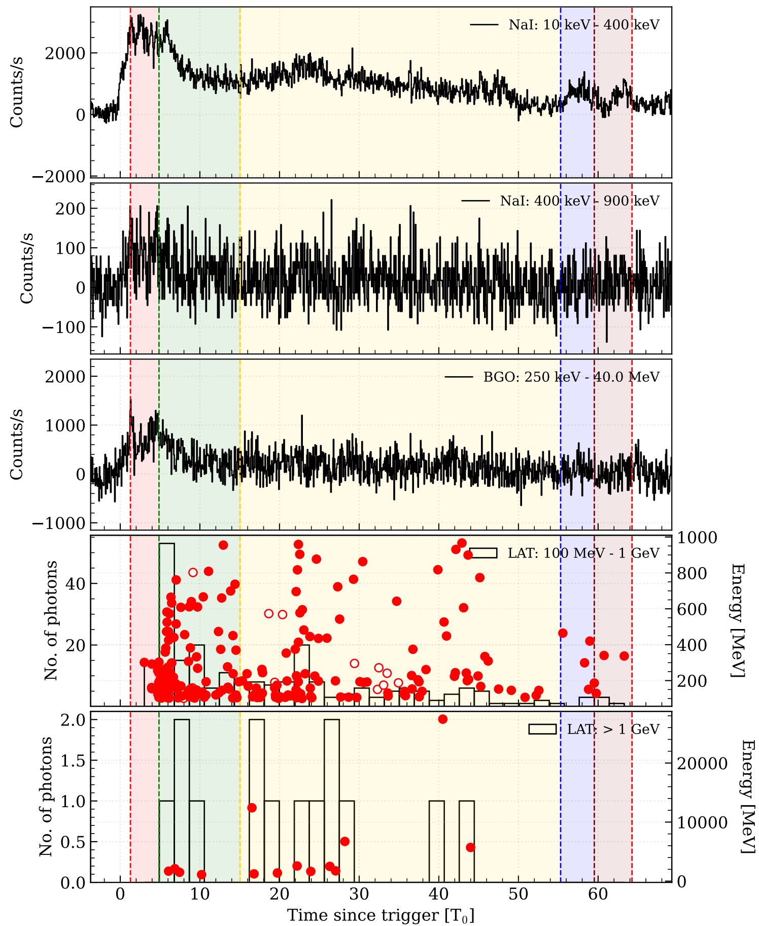
GRB080916C
