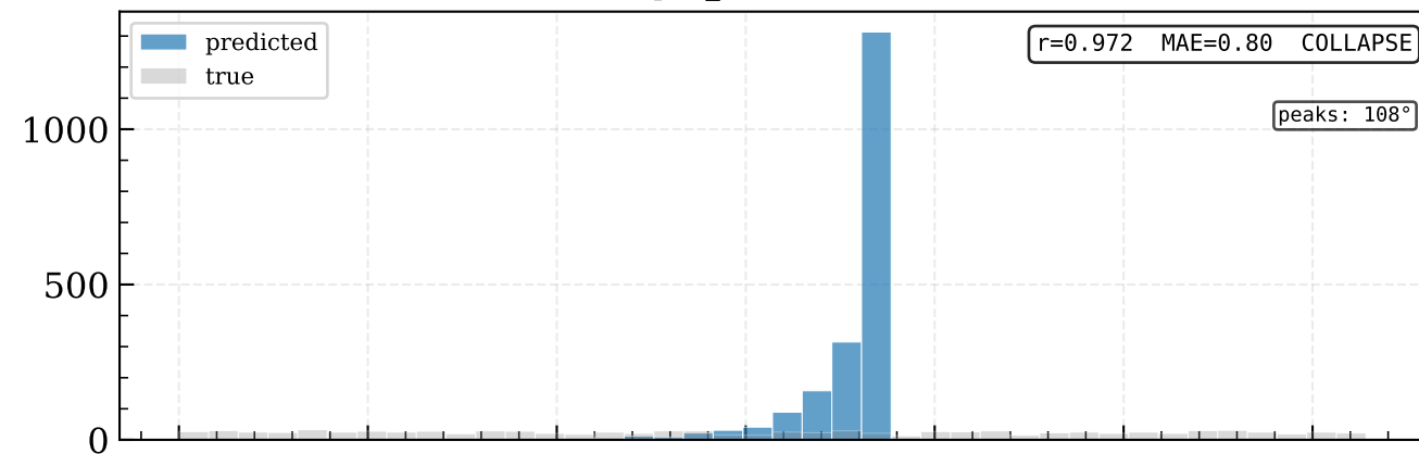
poc_a (baseline)
