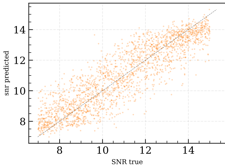
poc_b (PoC) R^2=0.789 MAE=0.824
