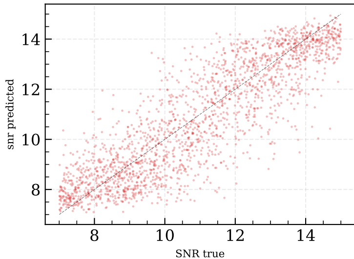
cnn_attention R^2=0.741 MAE=0.893
