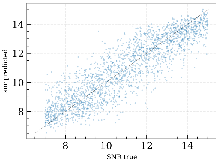
poc_a (baseline) R^2=0.787 MAE=0.824
