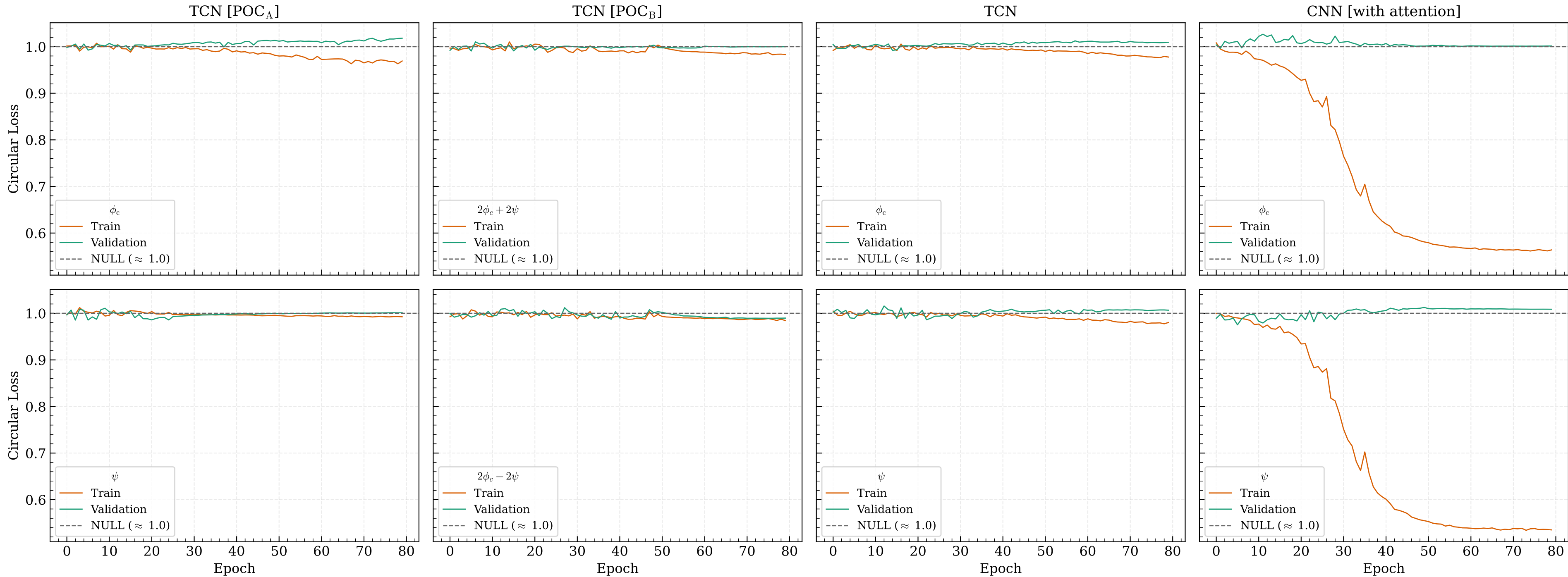
Train vs. Validation Circular Loss — Down-Select-Confirmed 4-Model Set (Redo) No model is null-certified here (Step 0 gate never cleared) — shown uniformly, not restricted
