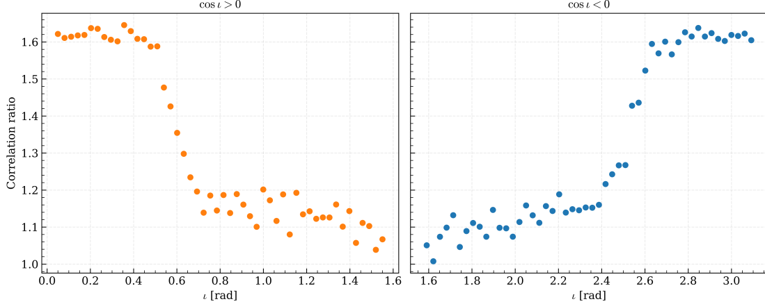
Figure 1: Analytic check of the corrected 2\varphi_c - 2\psi degeneracy structure: ratio of the strain correlation with the well-constrained combination to the poorly-constrained one, as a function of inclination.
