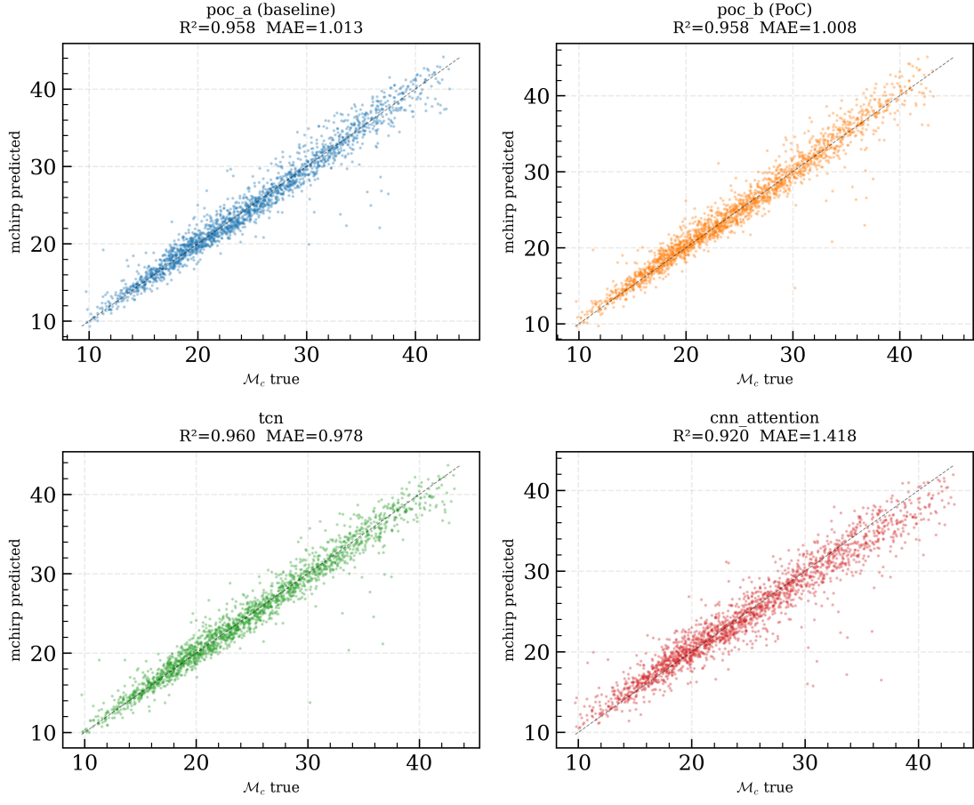
Figure 2: Positive-control recovery (chirp mass) for the four down-selected models.
