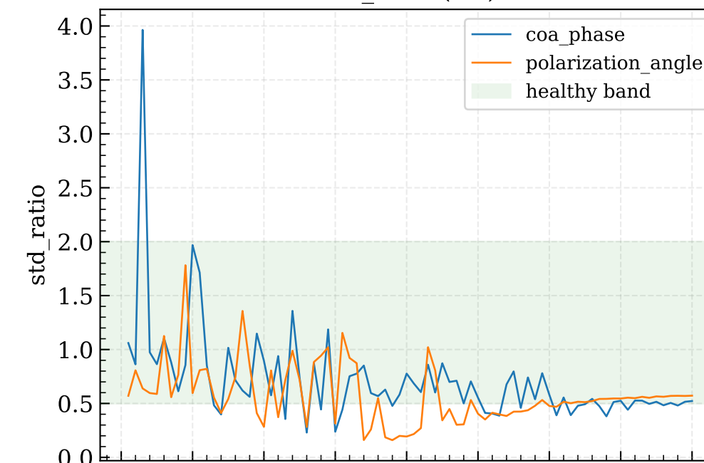
\lambda=0.05 (retune) [a] std_ratio (val)
