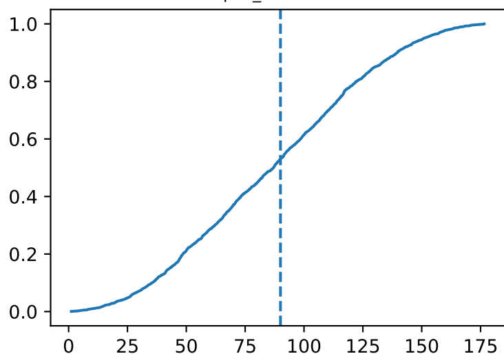
tcn — CDF
