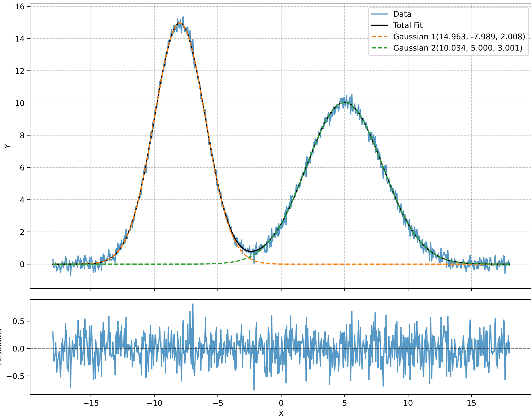
Fit and Residuals
