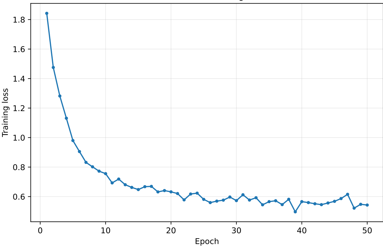
Swin-UNETR Training Loss
