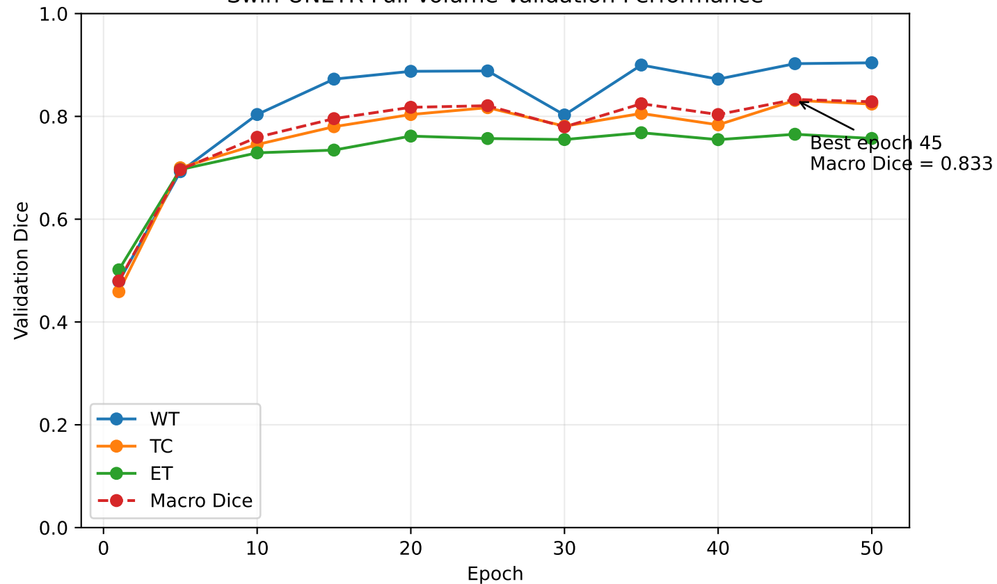
Swin-UNETR Full-Volume Validation Performance
