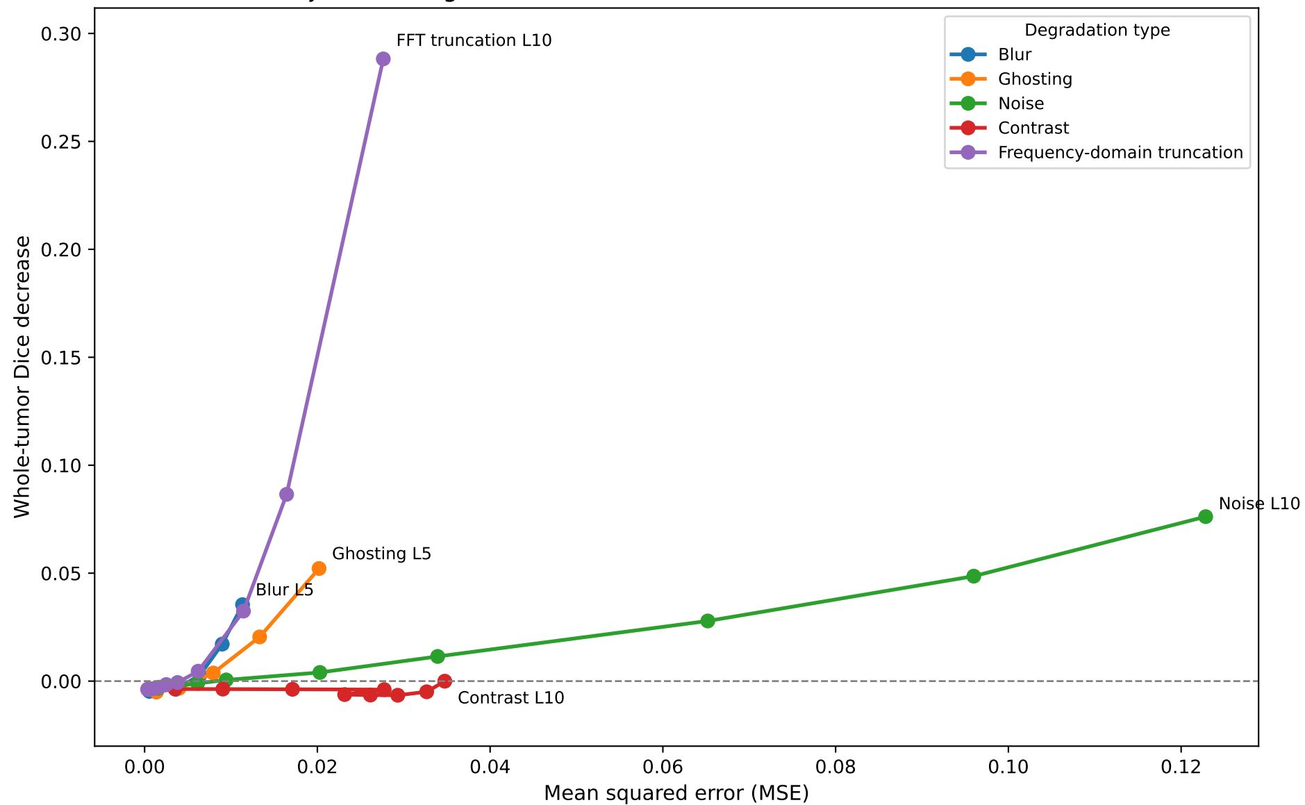
Objective Image Distortion Versus nnU-Net Whole-Tumor Dice Loss
