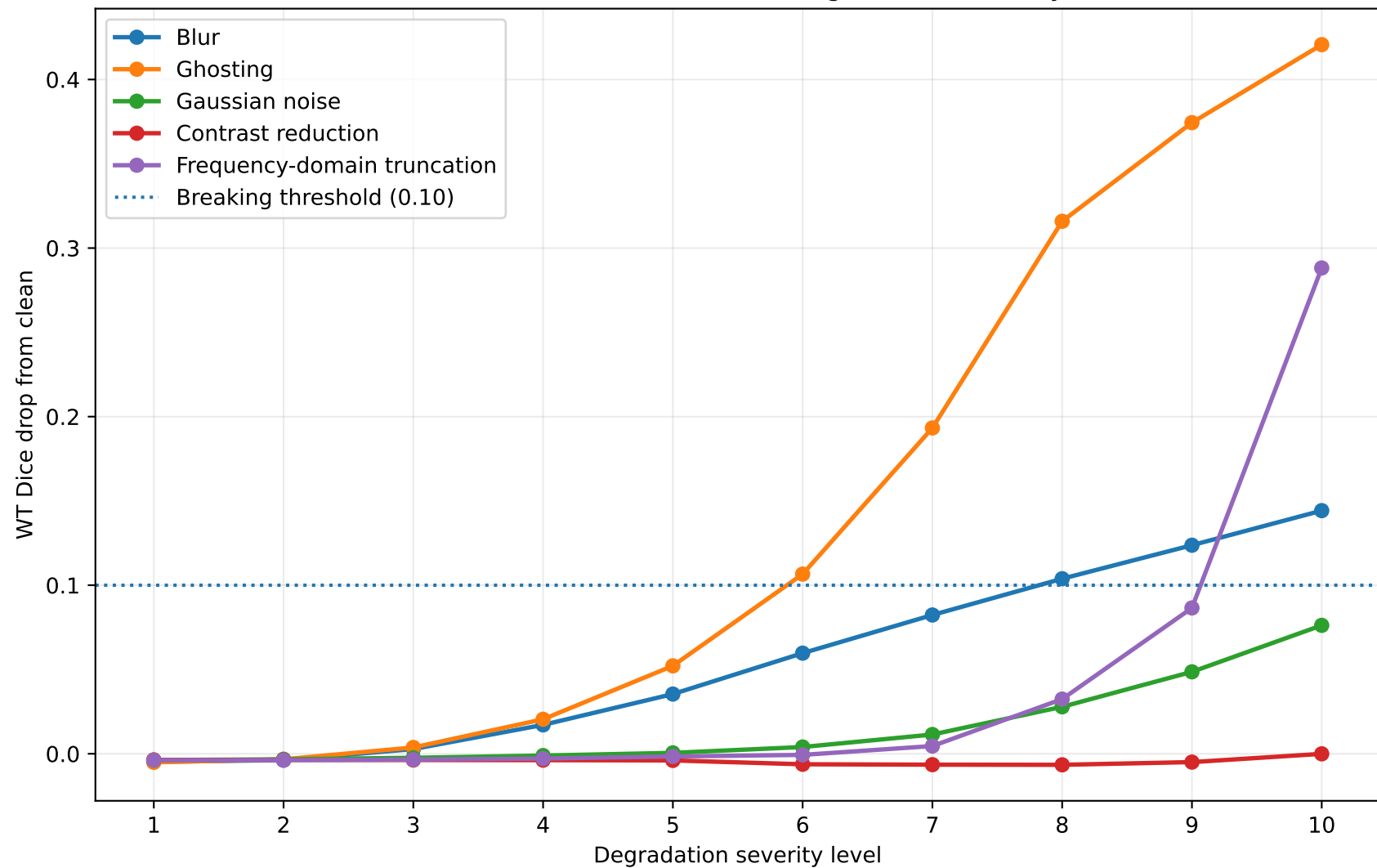
nnU-Net WT Dice loss across degradation severity
