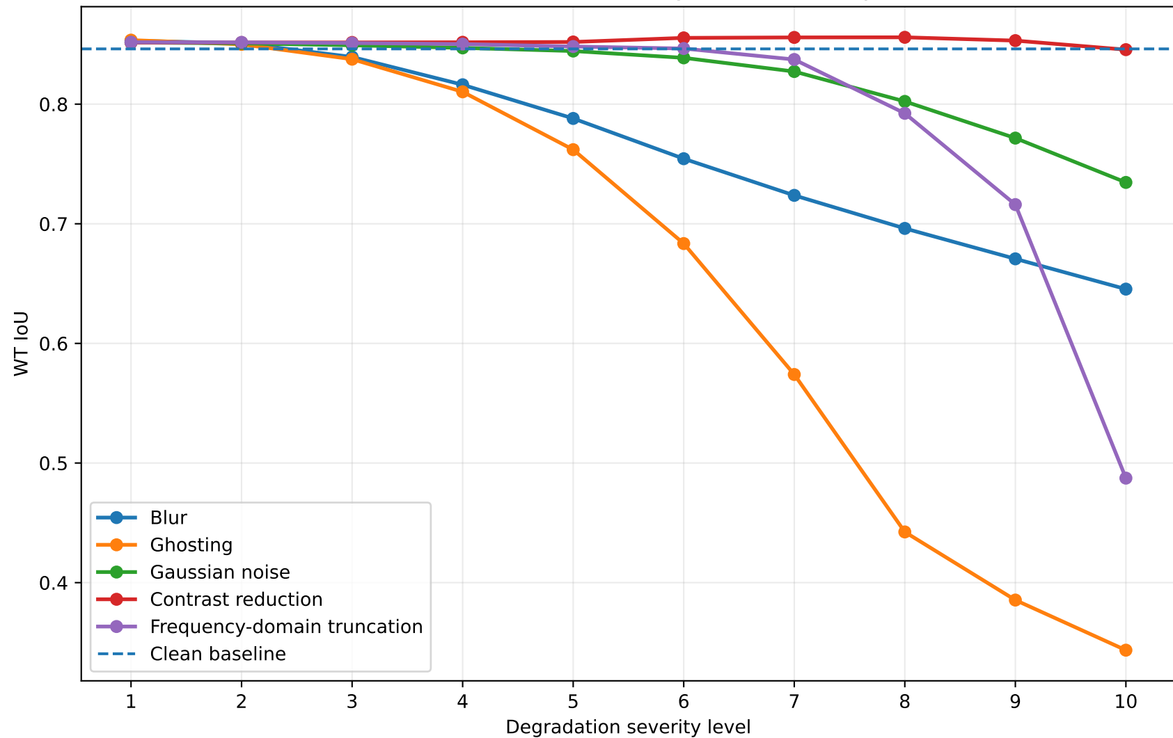
nnU-Net WT IoU across degradation severity
