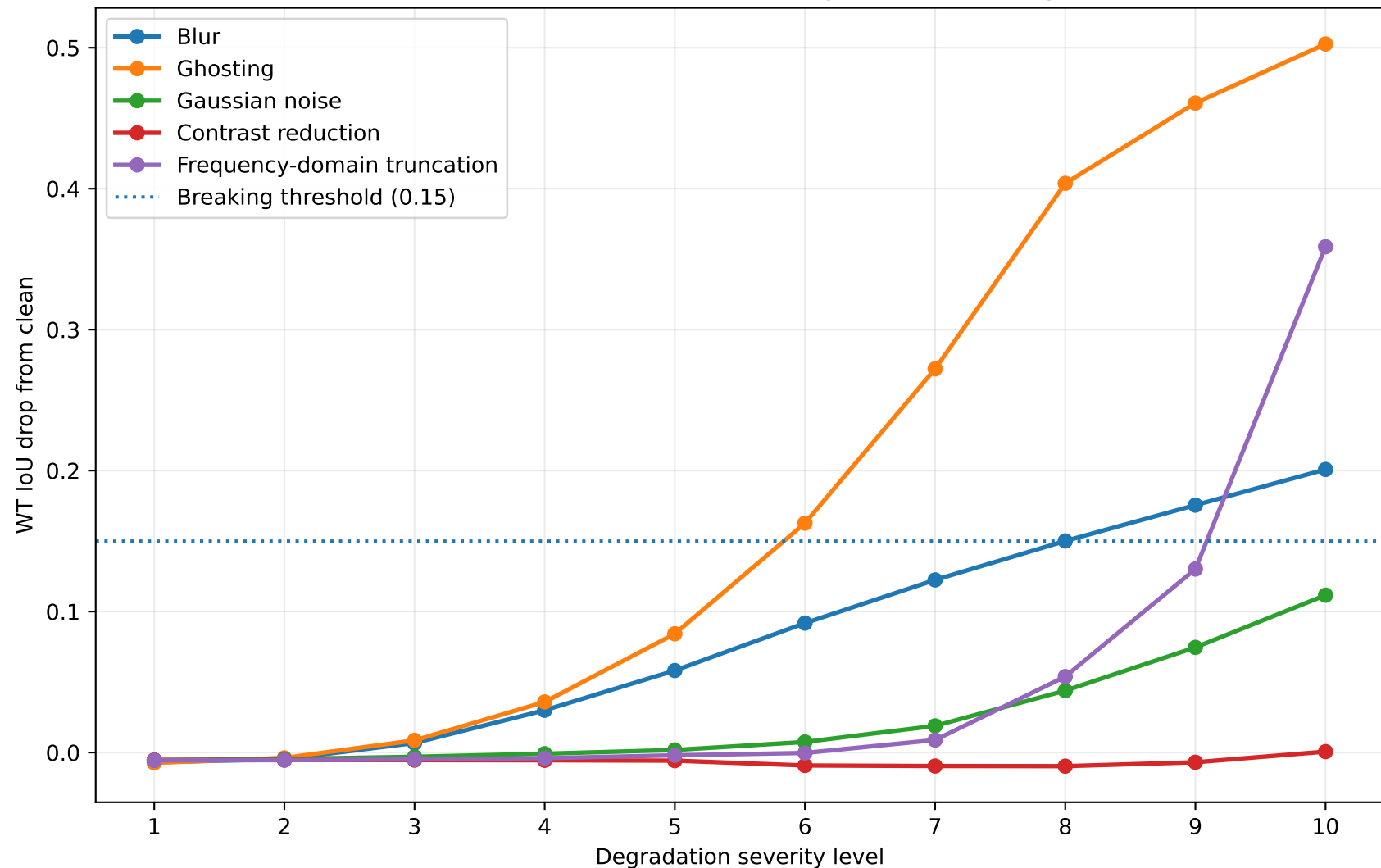
nnU-Net WT IoU loss across degradation severity
