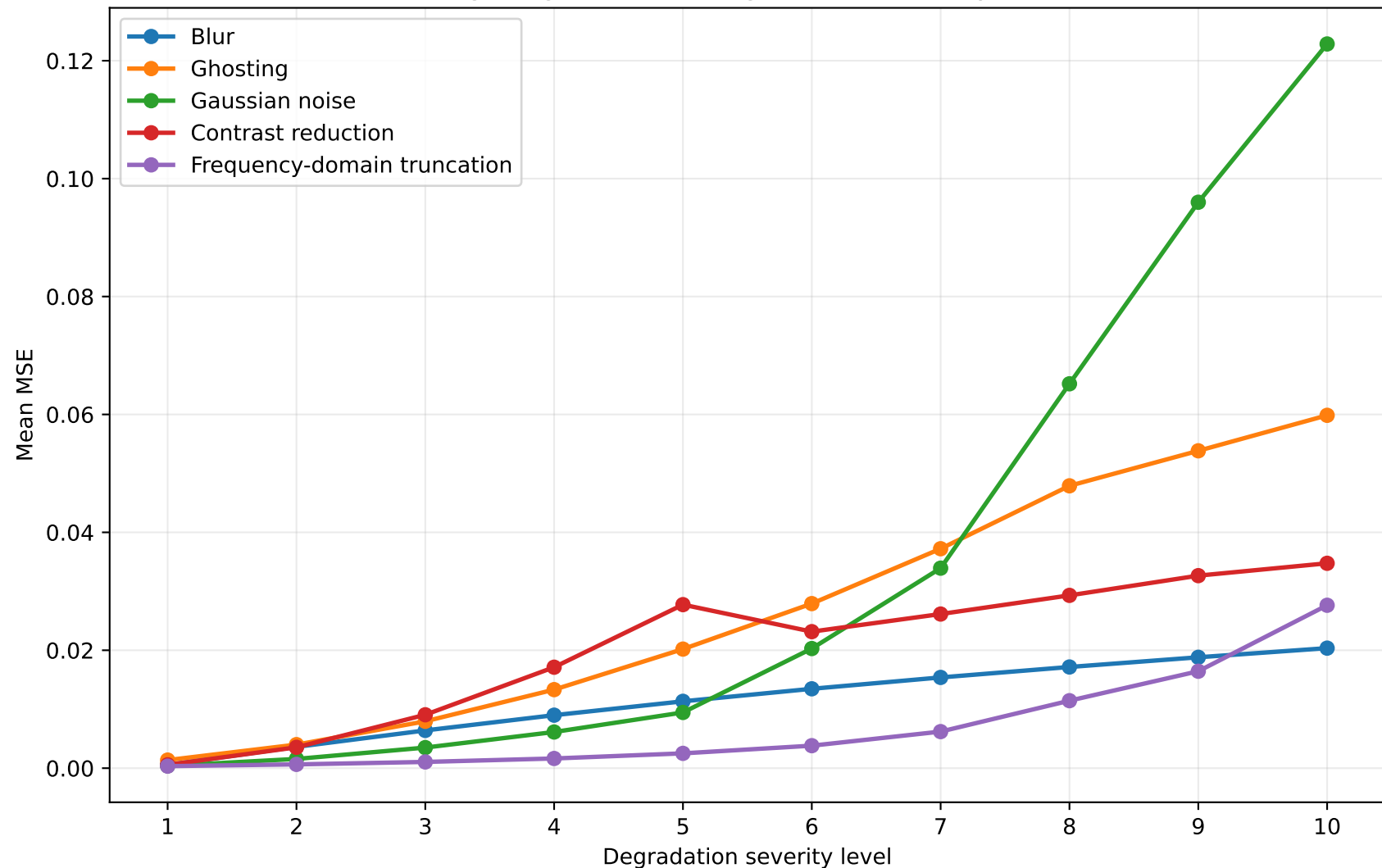
Image degradation strength across severity levels
