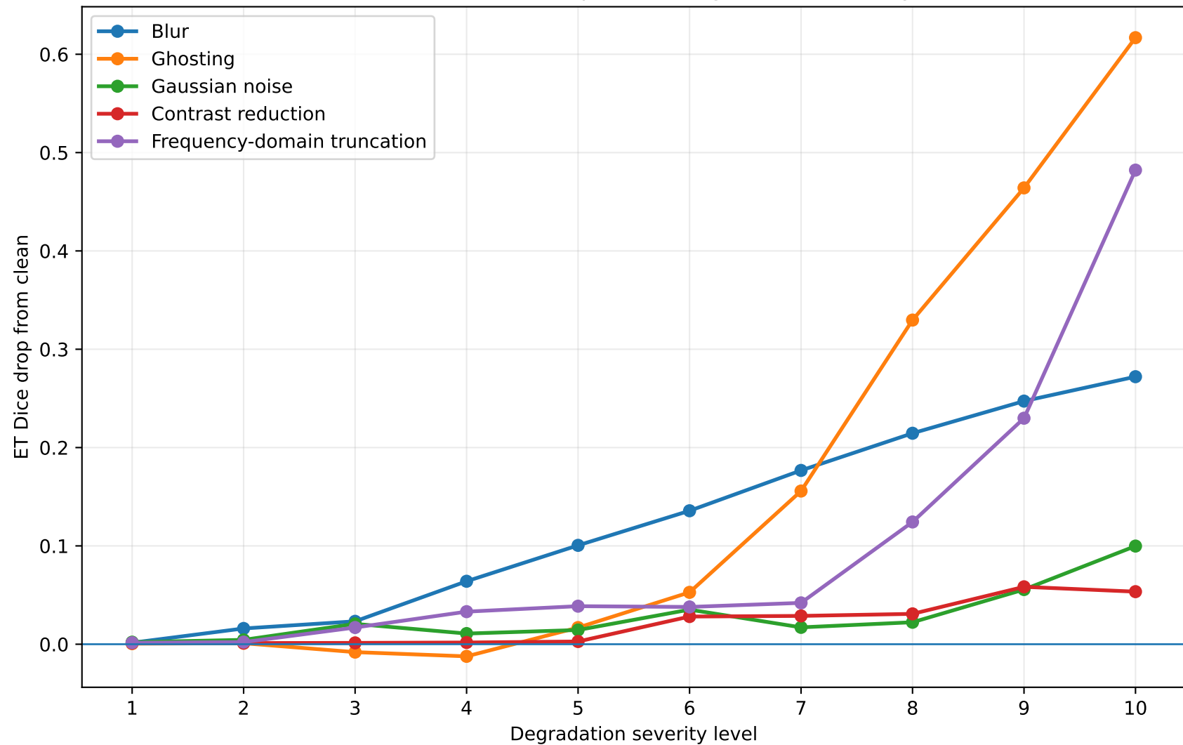
nnU-Net ET Dice drop across degradation severity
