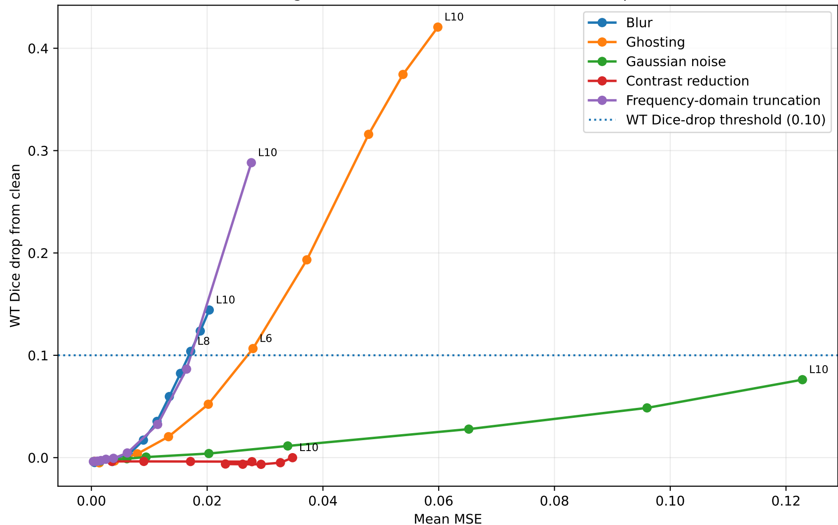
Image distortion versus nnU-Net WT Dice drop
