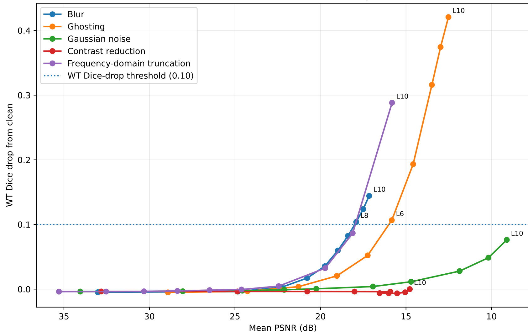
PSNR versus nnU-Net WT Dice drop
