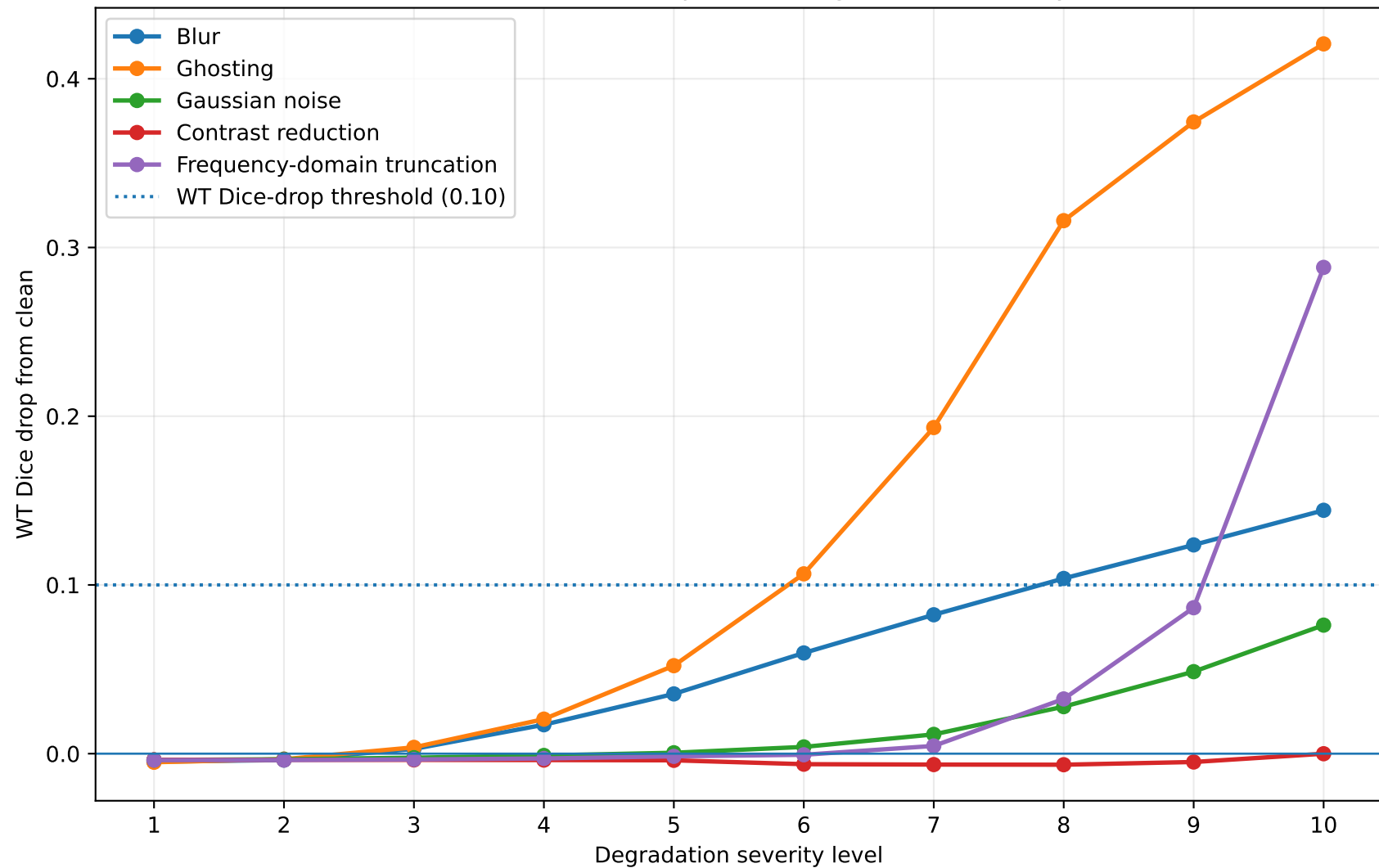
nnU-Net WT Dice drop across degradation severity
