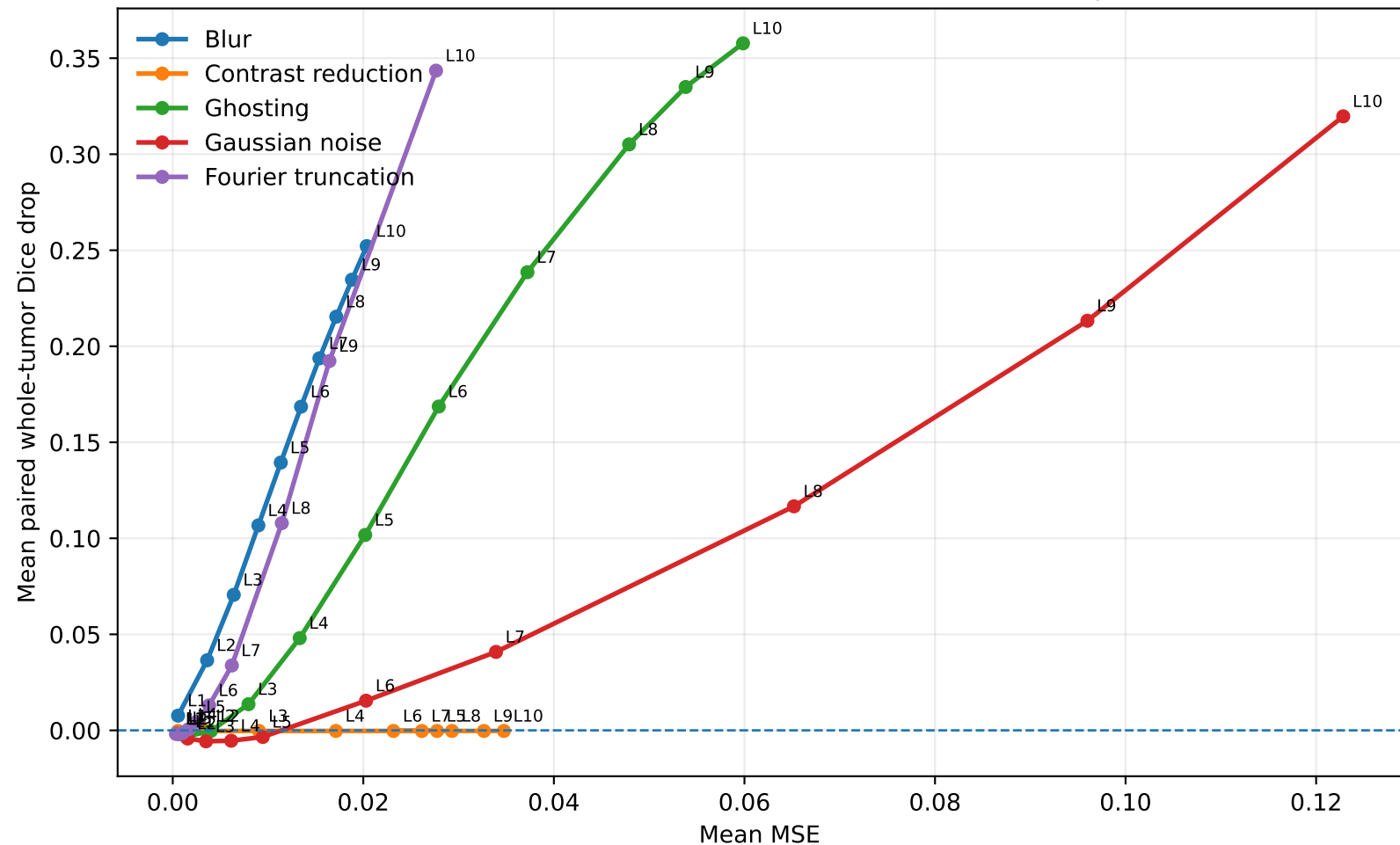
Custom 3D U-Net: MSE vs Whole-Tumor Dice Drop
