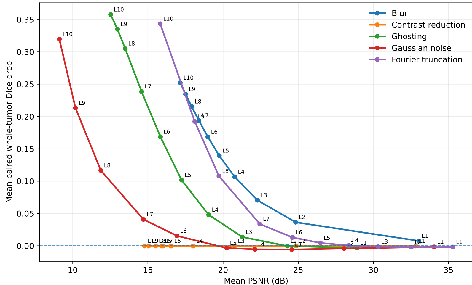
Custom 3D U-Net: PSNR vs Whole-Tumor Dice Drop
