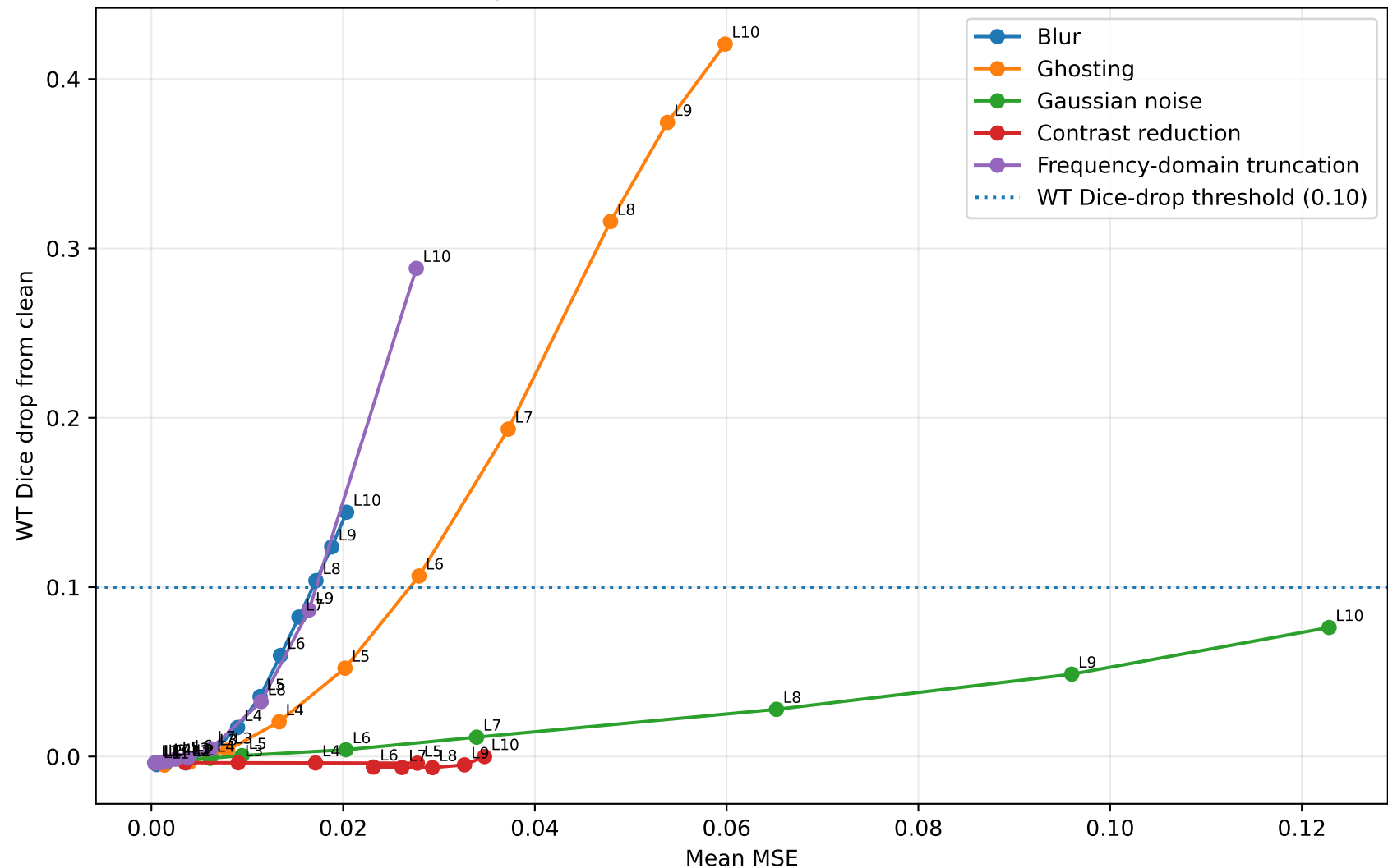
Image distortion versus nnU-Net WT Dice loss
