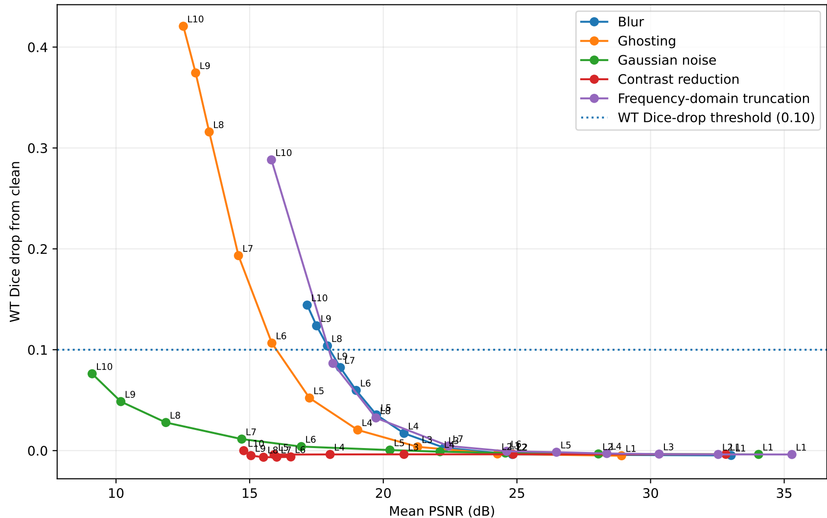
PSNR versus nnU-Net WT Dice loss
