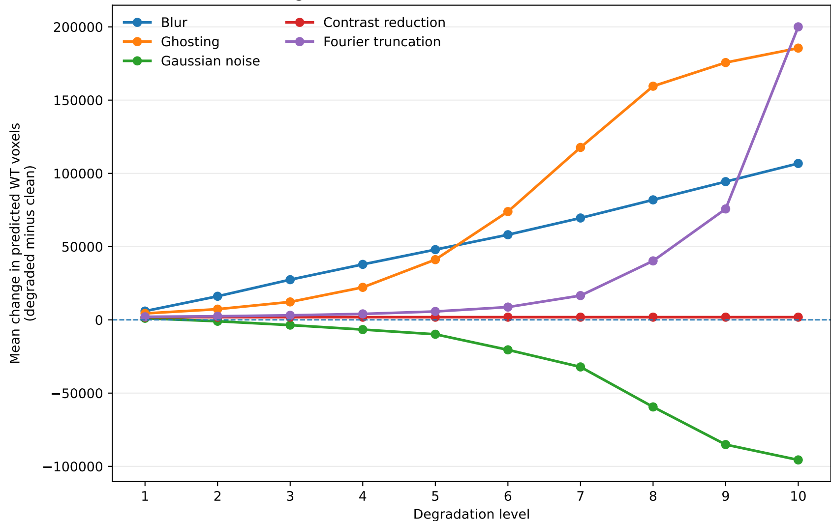
Change in Swin-UNETR Whole-Tumor Prediction Volume
