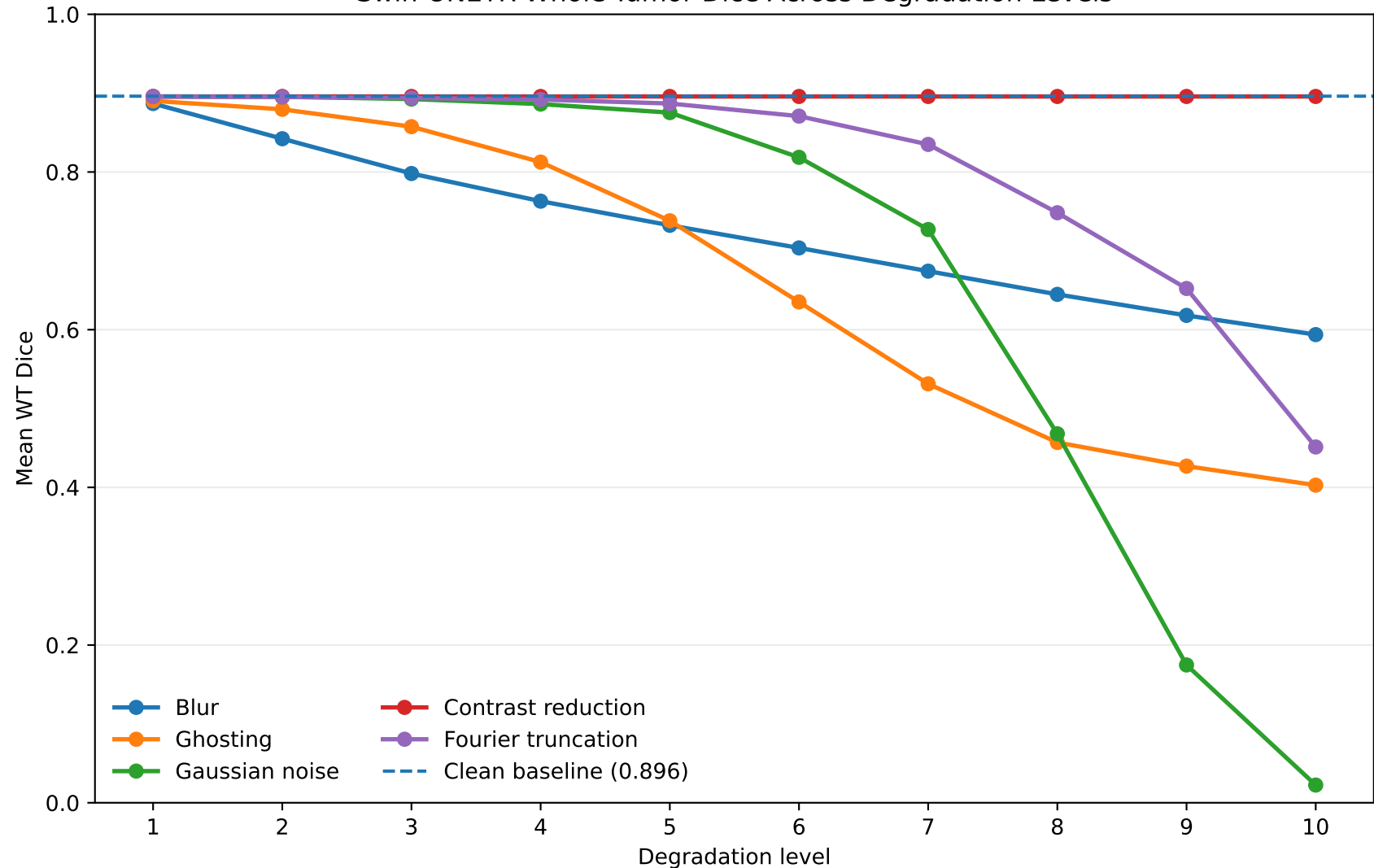
Swin-UNETR Whole-Tumor Dice Across Degradation Levels
