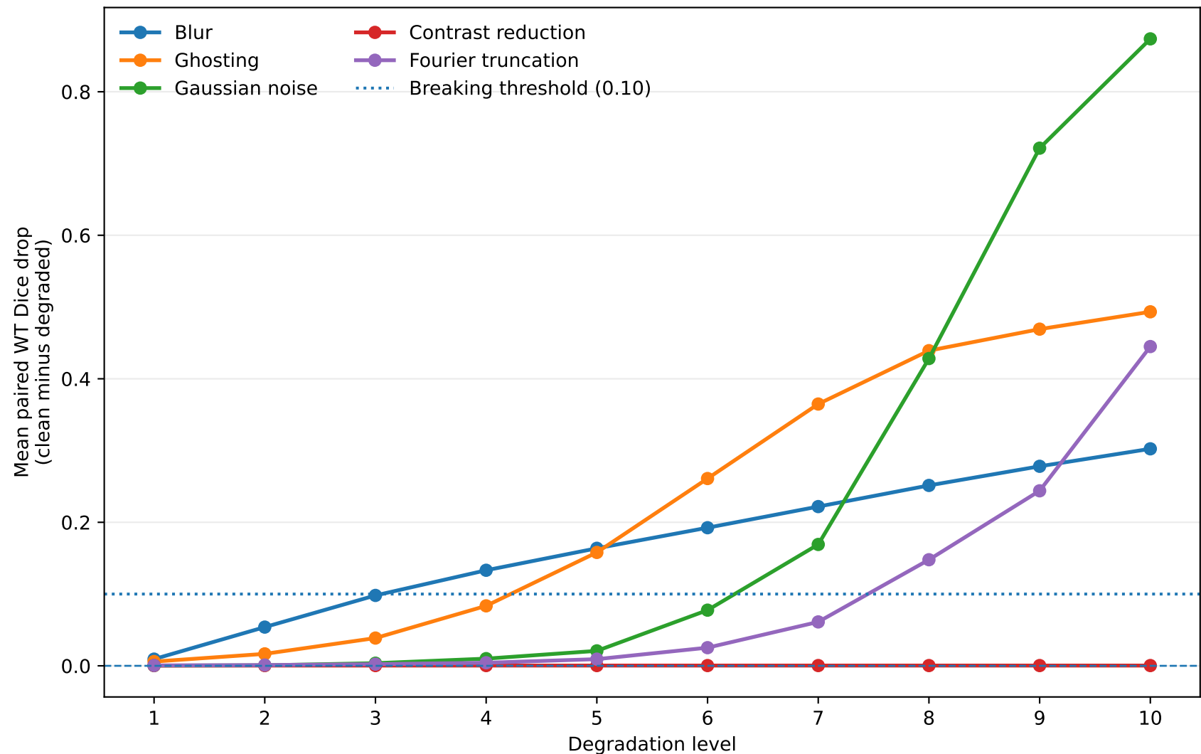
Swin-UNETR Whole-Tumor Dice Decrease
