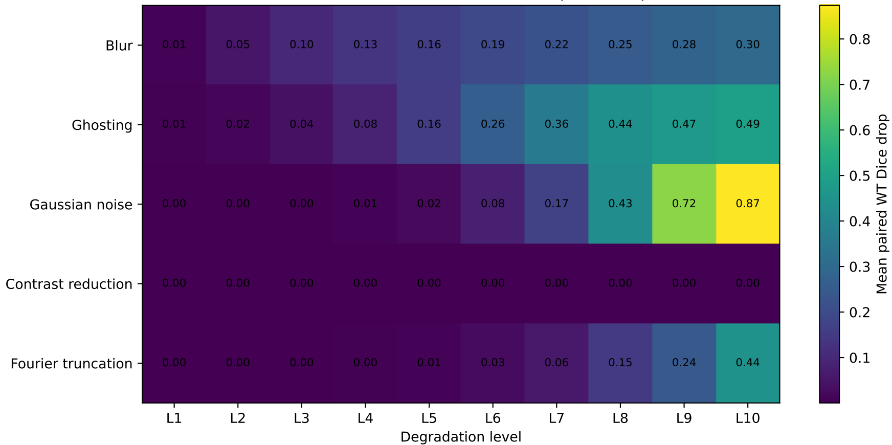
Swin-UNETR Whole-Tumor Dice-Drop Heatmap
