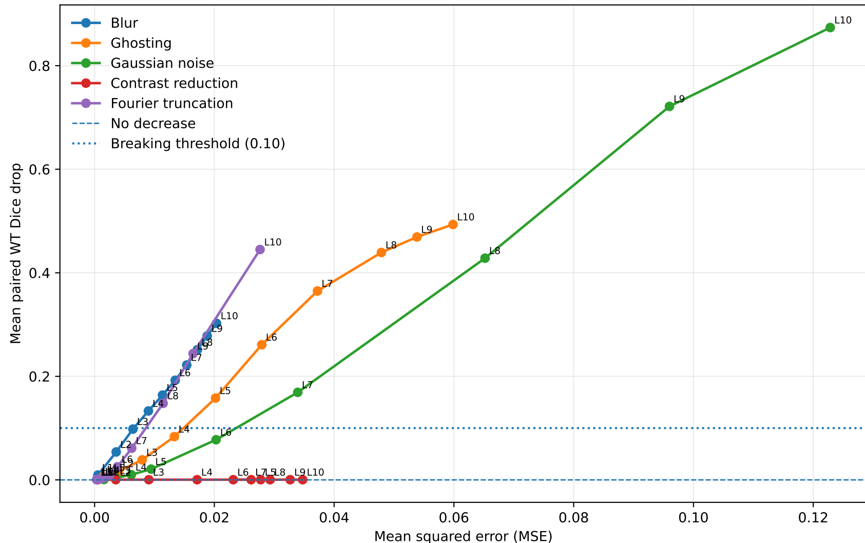
Swin-UNETR: MSE versus WT Dice decrease
