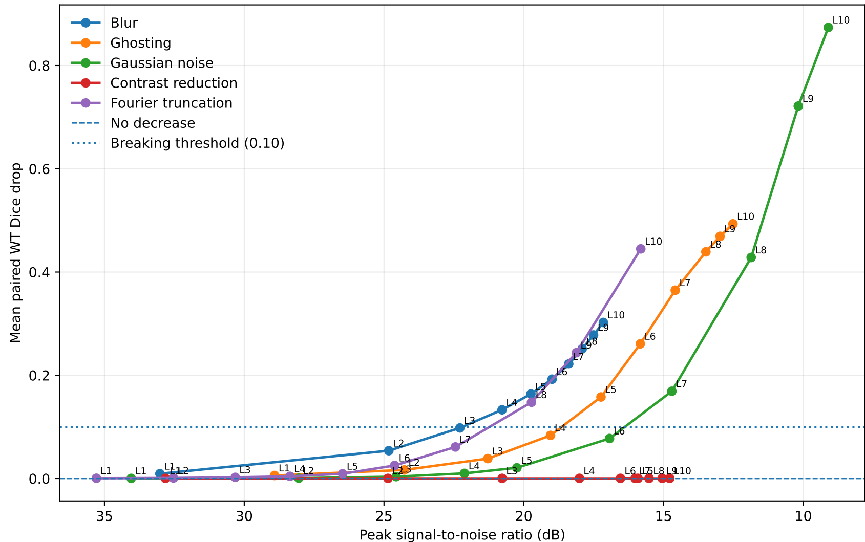
Swin-UNETR: PSNR versus WT Dice decrease
