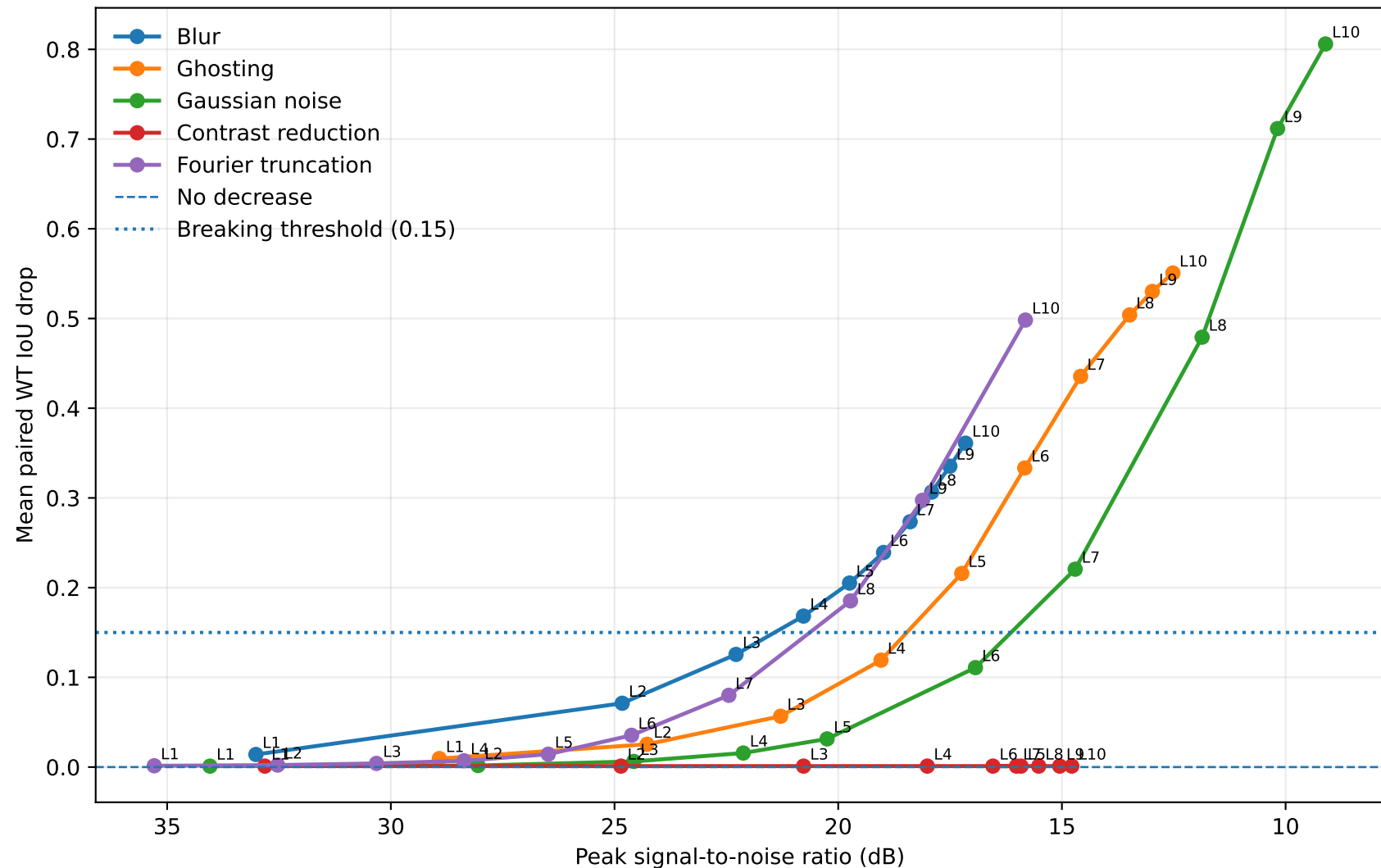
Swin-UNETR: PSNR versus WT IoU decrease
