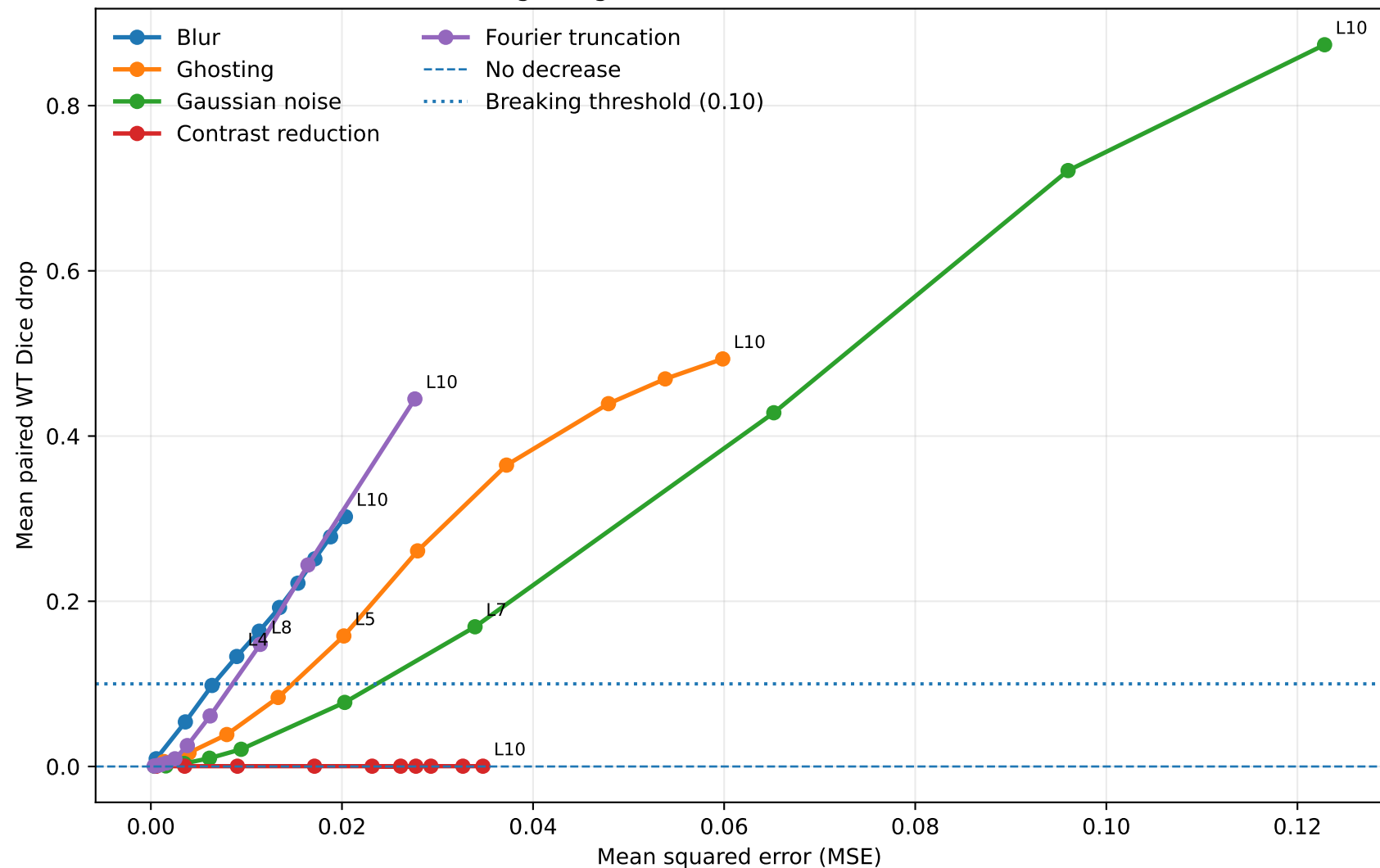
Swin-UNETR: Image Degradation versus Whole-Tumor Dice Decrease
