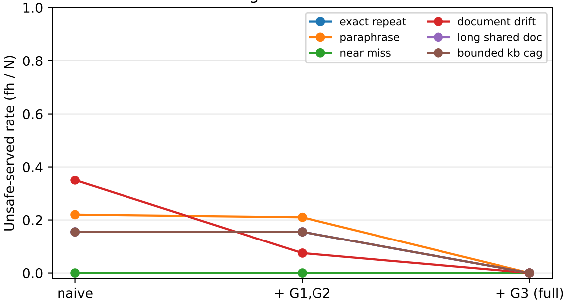
Cumulative gate-stack USR reduction
