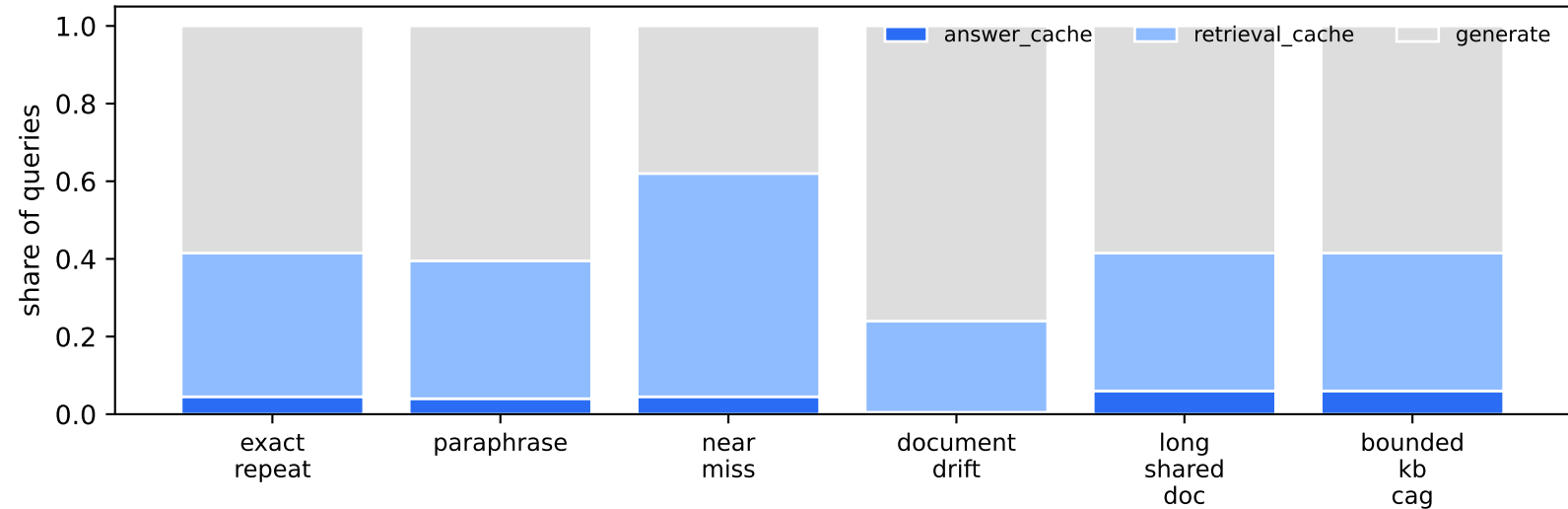
Path mix under GroundedCache (full)
