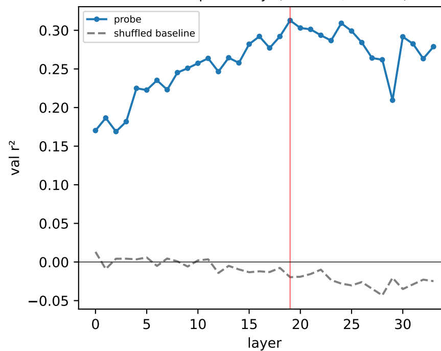
Others' Responsibility (best L19, r^2=0.31 )
