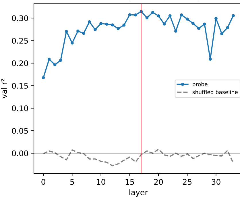
Suddenness (best L17, r^2=0.31 )
