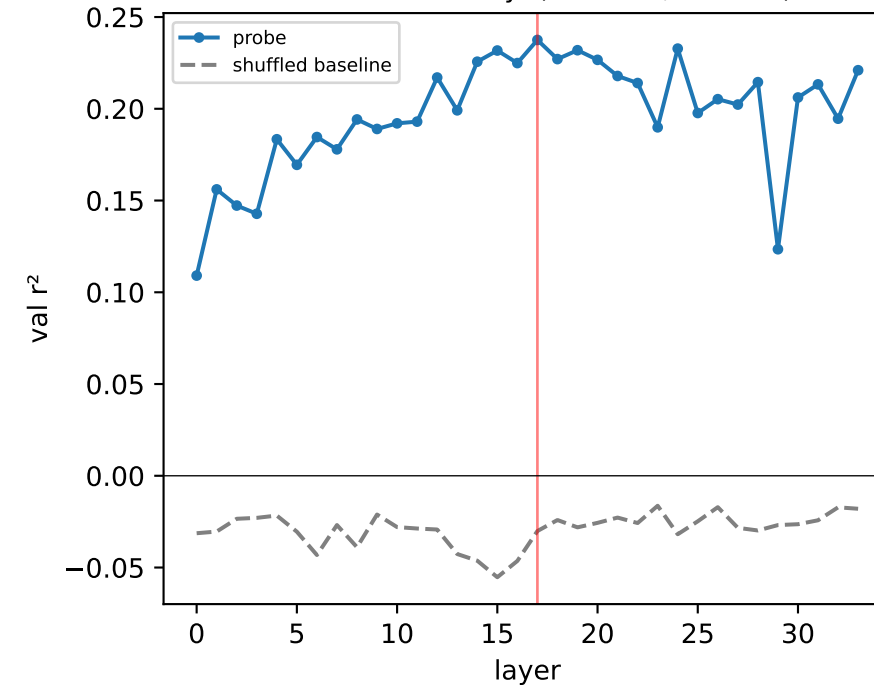
Event Predictability (best L17, r^2=0.24 )
