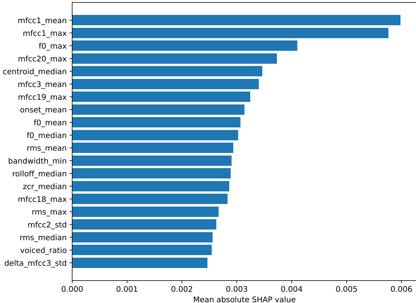
Global SHAP Feature Importance of Acoustic Branch
