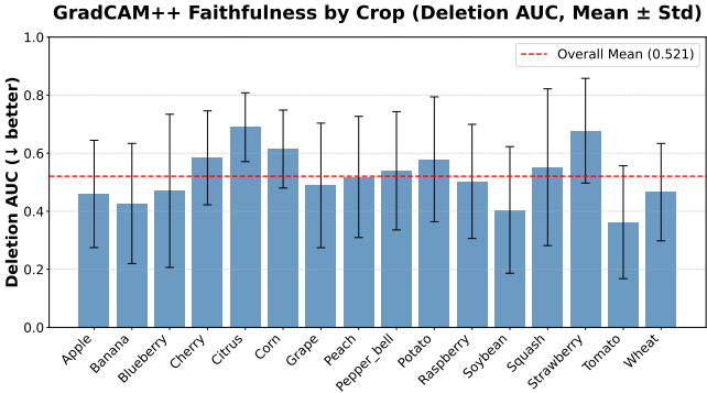
Fig. 6: Per-crop deletion AUC for GradCAM++ heatmaps across 678 test samples.
