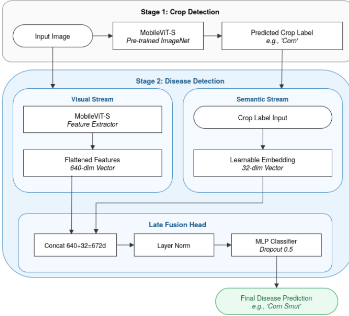
Fig. 2: Overview of the two-stage architecture, demonstrating the fusion of crop predictions with visual features.
