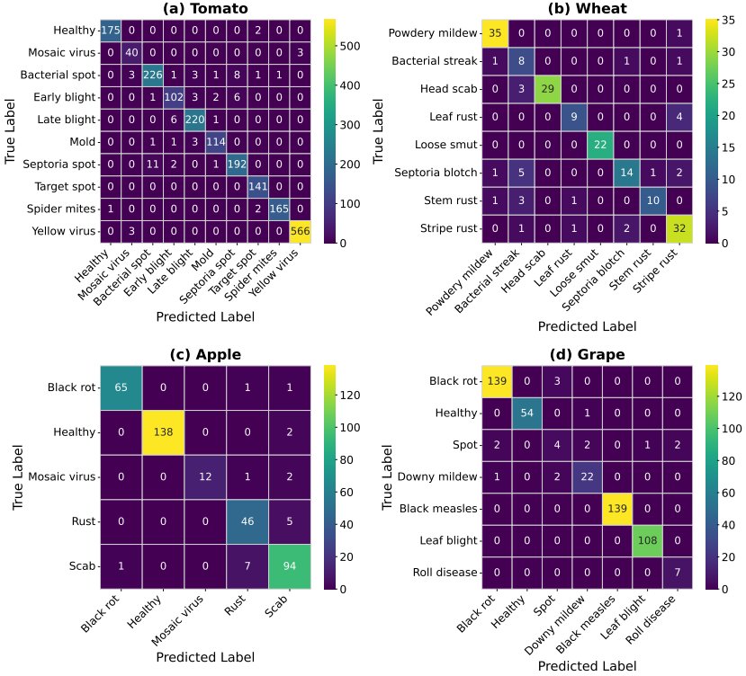
Fig. 4: Confusion matrices of four crops: Tomato, Wheat, Apple, and Grape.
