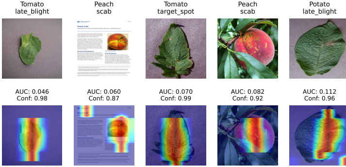
Fig. 5: Top row: original images. Bottom row: GradCAM++ overlays with deletion AUC and confidence scores.
