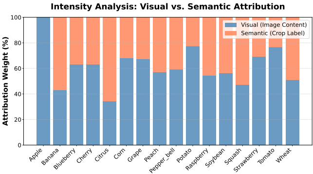
Fig. 7: Per-crop visual vs. semantic attribution split. Crops with high semantic reliance (citrus, banana, squash, wheat) are predominantly sourced from in-the-wild datasets; visually dominant crops (tomato, potato, apple) are largely PlantVillage-sourced.
