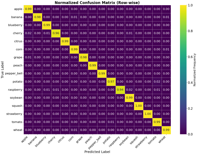
Fig. 3: Confusion matrix for crop detection.
