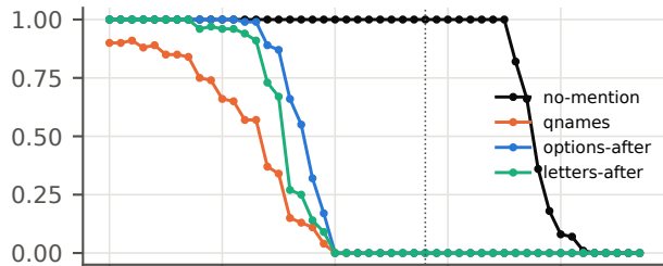
ID sweep, Qwen2.5-14B
