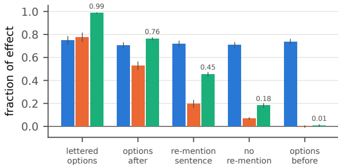
Mistral-Small-24B
