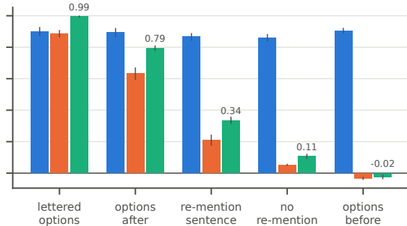
Qwen2.5-72B
