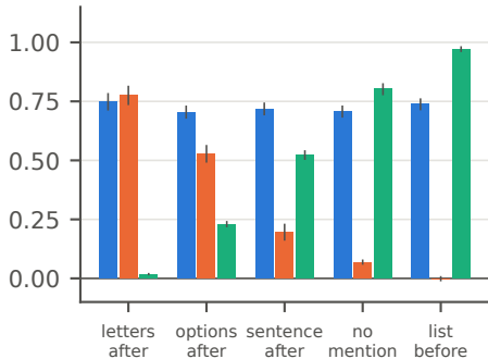
(a) Mistral-Small-24B
