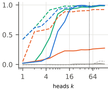
Mistral-7B, sentence-after
