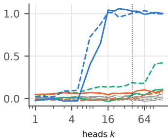
Qwen2.5-7B, sentence-after
