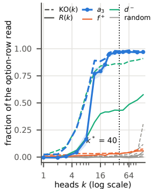
(b) heads: Qwen2.5-7B
