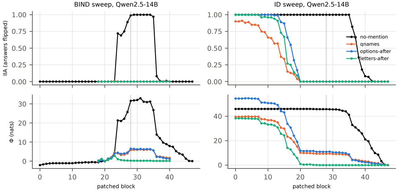
Figure 7. Sweeps of the two edits over the patched block (Qwen2.5-14B-Instruct, 150 pairs, BF16). Top: IIA, the fraction of answers flipped to the target; bottom: \Phi , the mean shift of m = \log p(\text{target}) - \log p(\text{queried drink}) . Left: the binding swap BIND (swept over blocks 18–40 in the formats that name candidates); right: the identity edit ID. Dotted: block \ell^* = 28 . \ell^* and \ell_{\text{ID}}^* are chosen on the NO-MENTION sweeps (preregistered); the other formats are reported.
