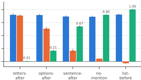
Qwen2.5-72B
