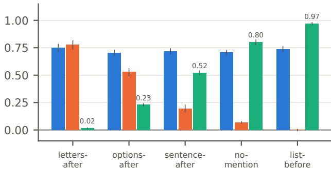
Mistral-Small-24B
