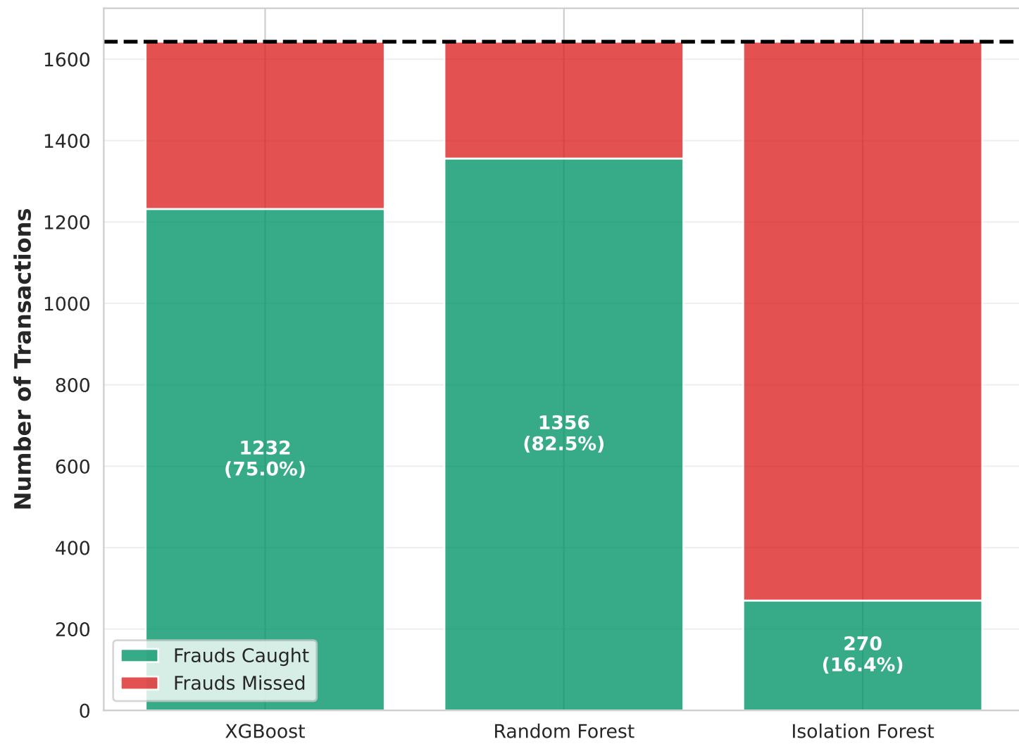
Fraud Detection Rate
