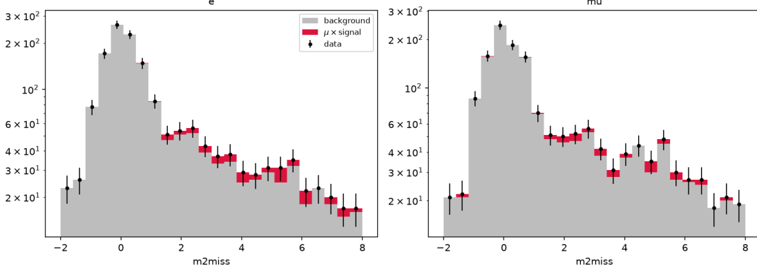
Figure 12: Post-fit m_{\text{miss}}^2 distributions of the projection re-run at the nominal luminosity, reproducing Fig. 10 exactly.
