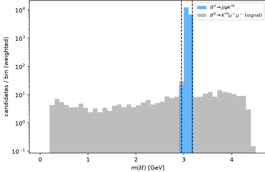
Figure 6: Dilepton mass m_{\ell\ell} in the muon channel after the K^* , M_{bc} and \Delta E requirements, stacked by sample (luminosity-weighted); the vertical lines mark the J/\psi veto window [2.946, 3.176] GeV.
