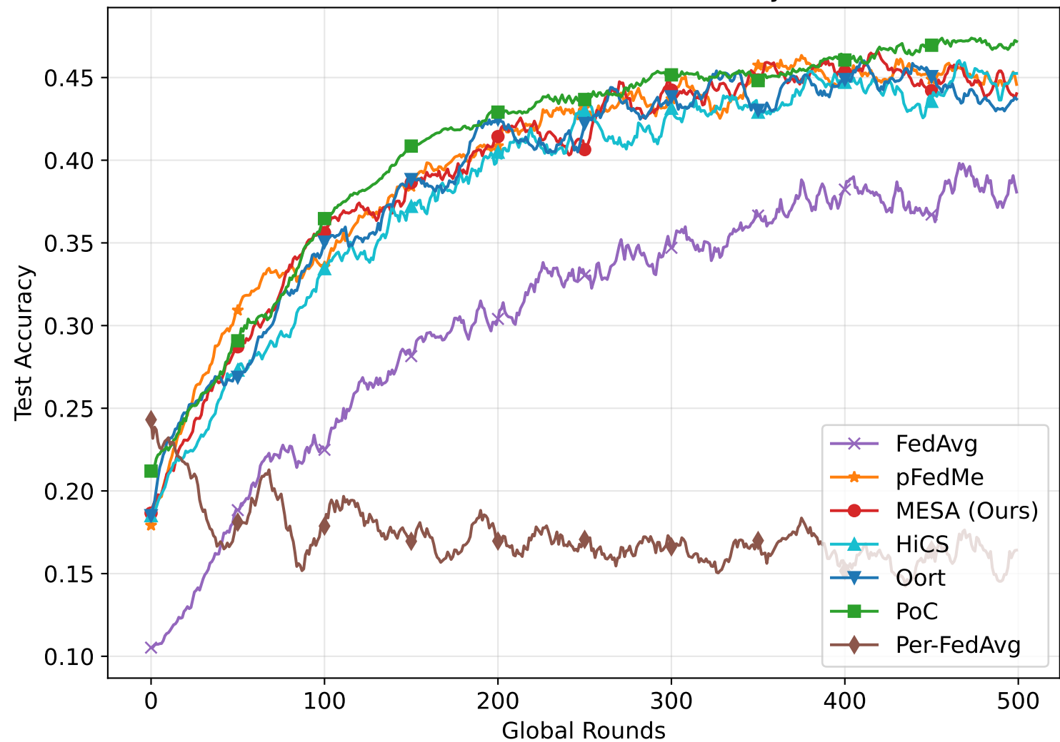
Cifar10 - CNN - Test Accuracy
