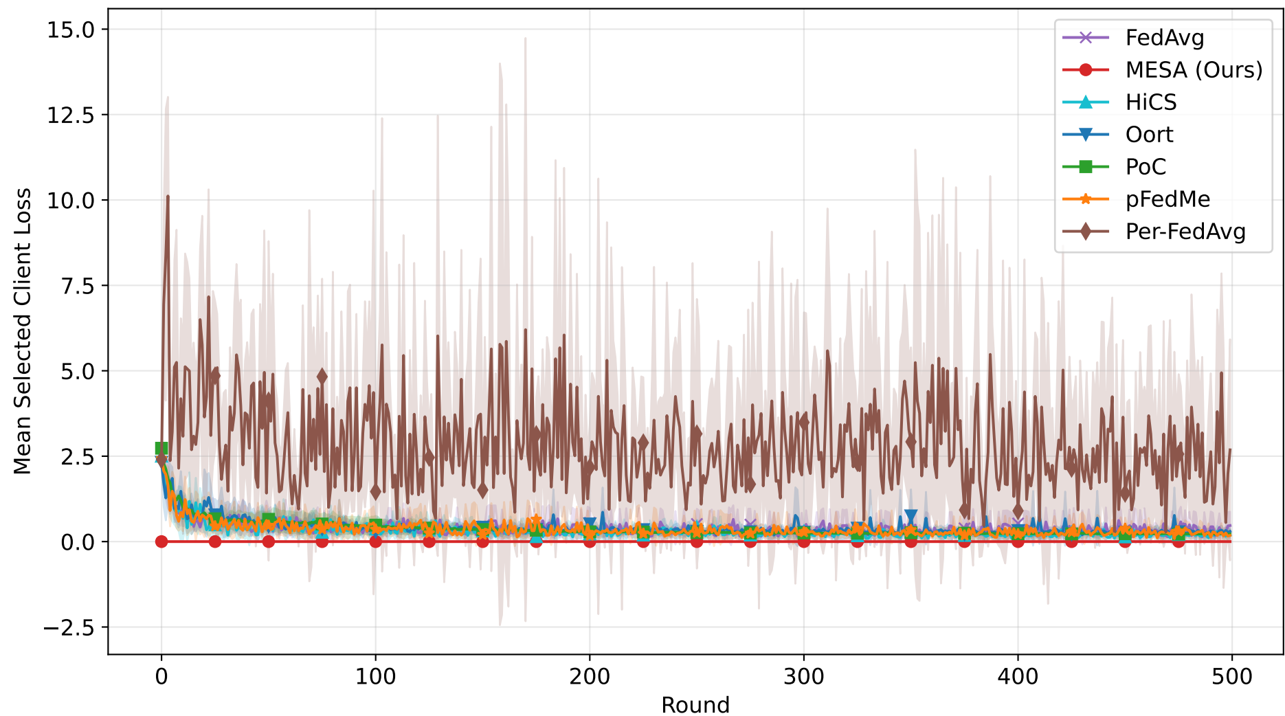
Mnist - MCLR - Selected Client Loss Over Rounds
