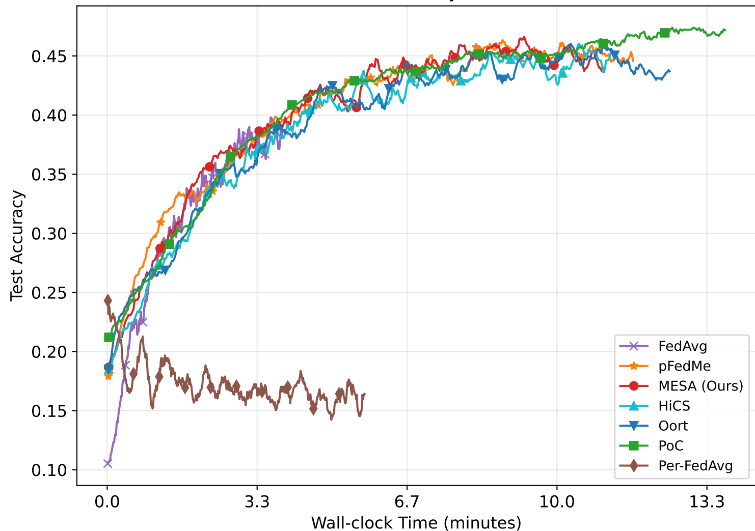
Cifar10 - CNN - Test Accuracy vs. Wall-clock Time
