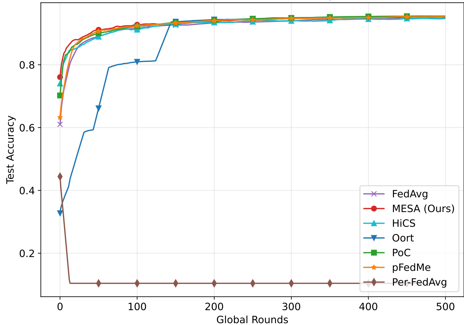
Mnist - DNN - Test Accuracy
