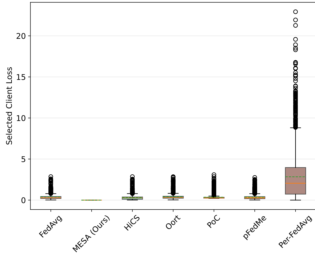
Box Plot of Selected Client Losses
