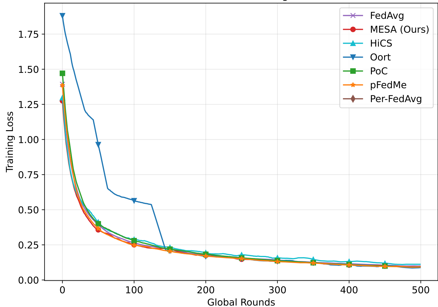
Mnist - DNN - Training Loss
