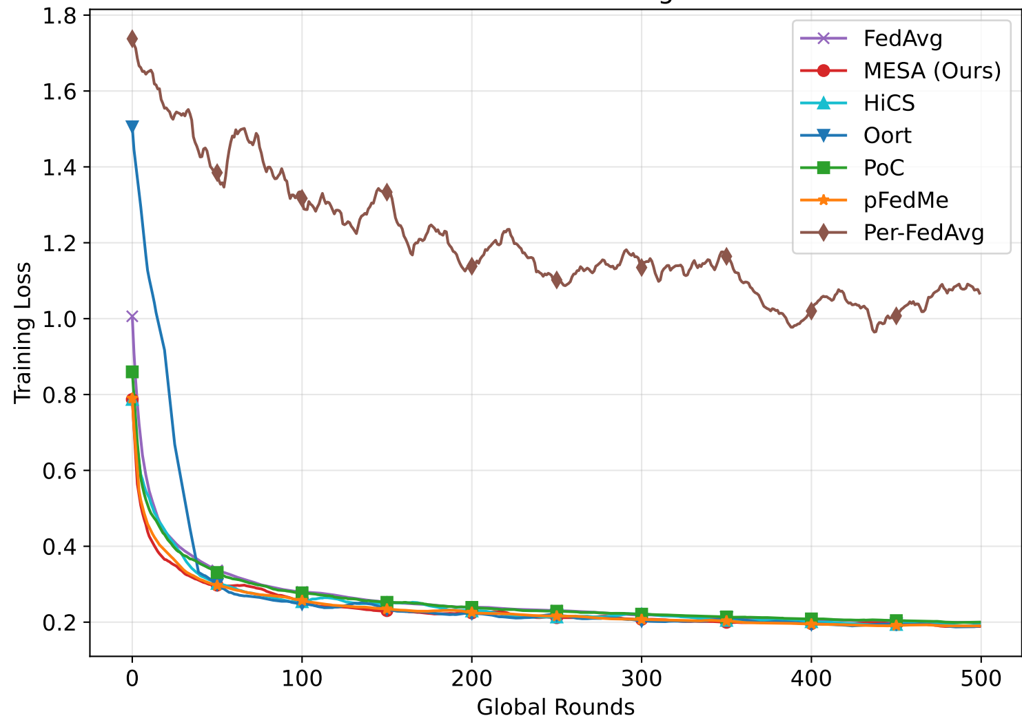
Mnist - MCLR - Training Loss
