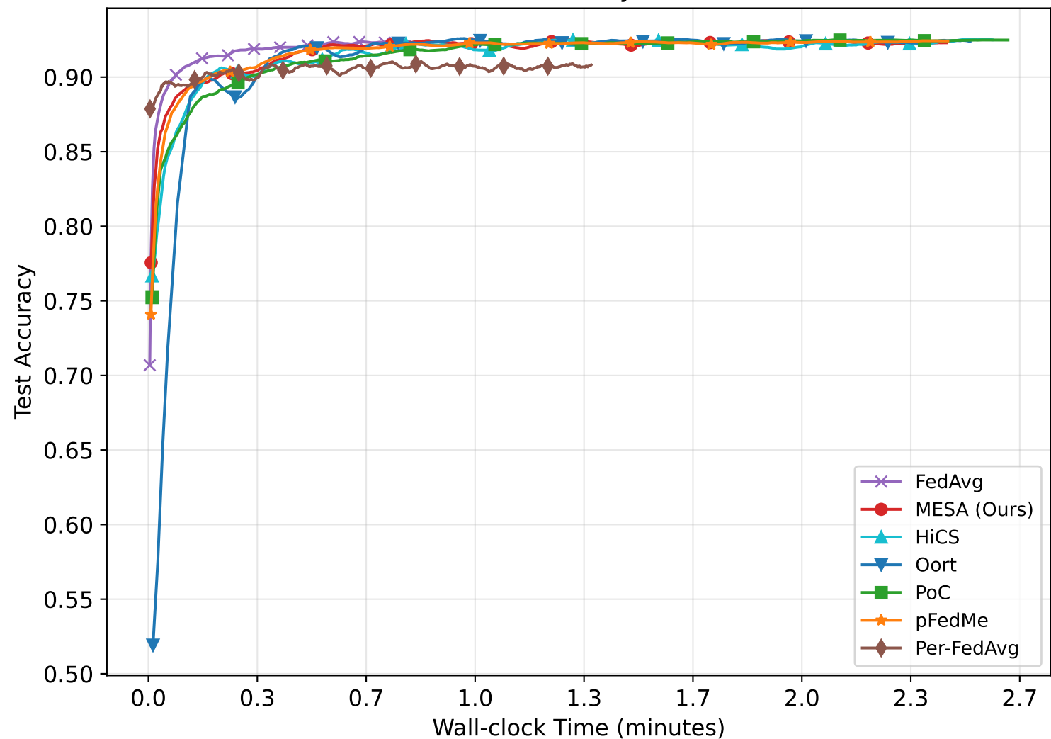
Mnist - MCLR - Test Accuracy vs. Wall-clock Time
