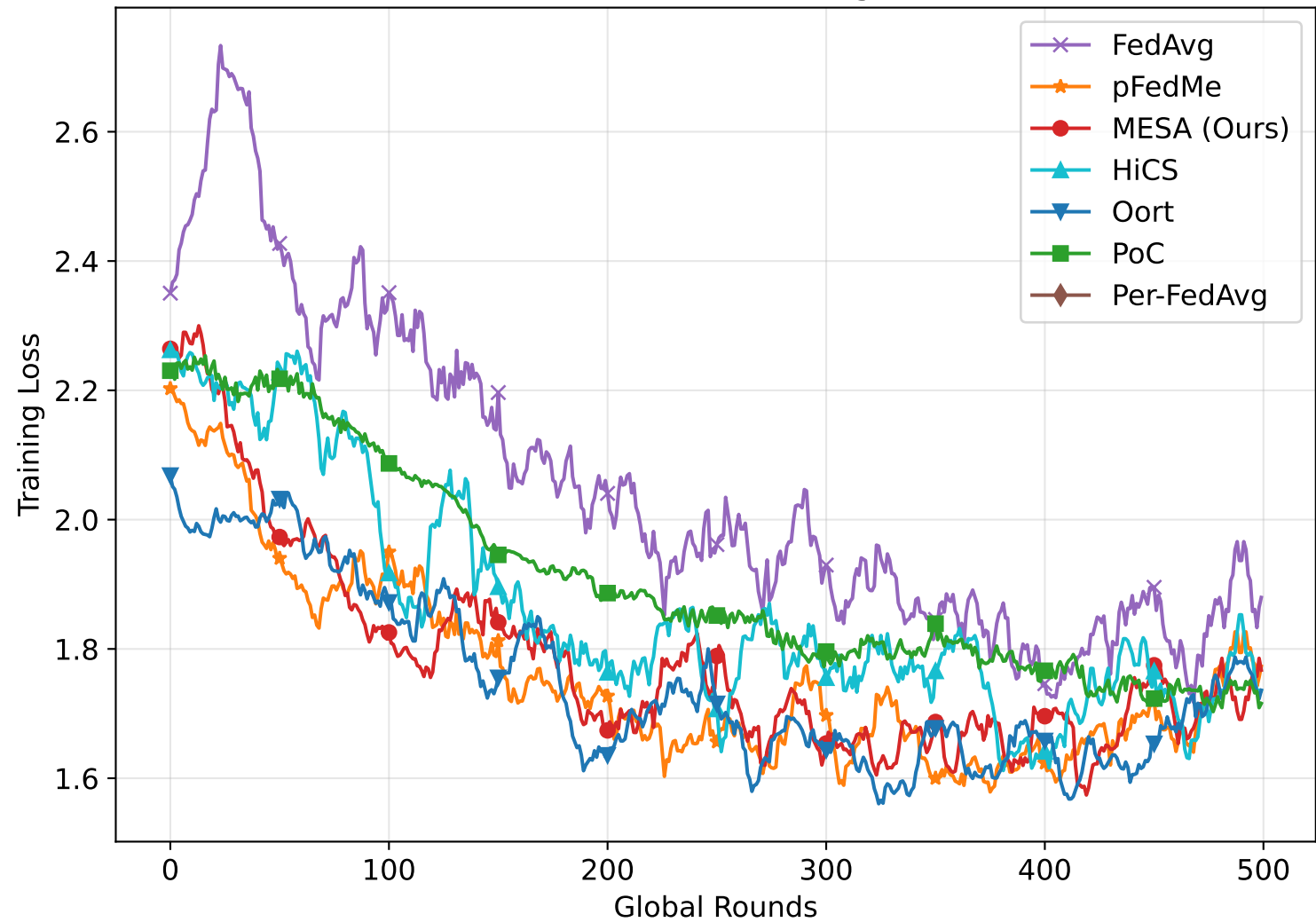
Cifar10 - CNN - Training Loss
