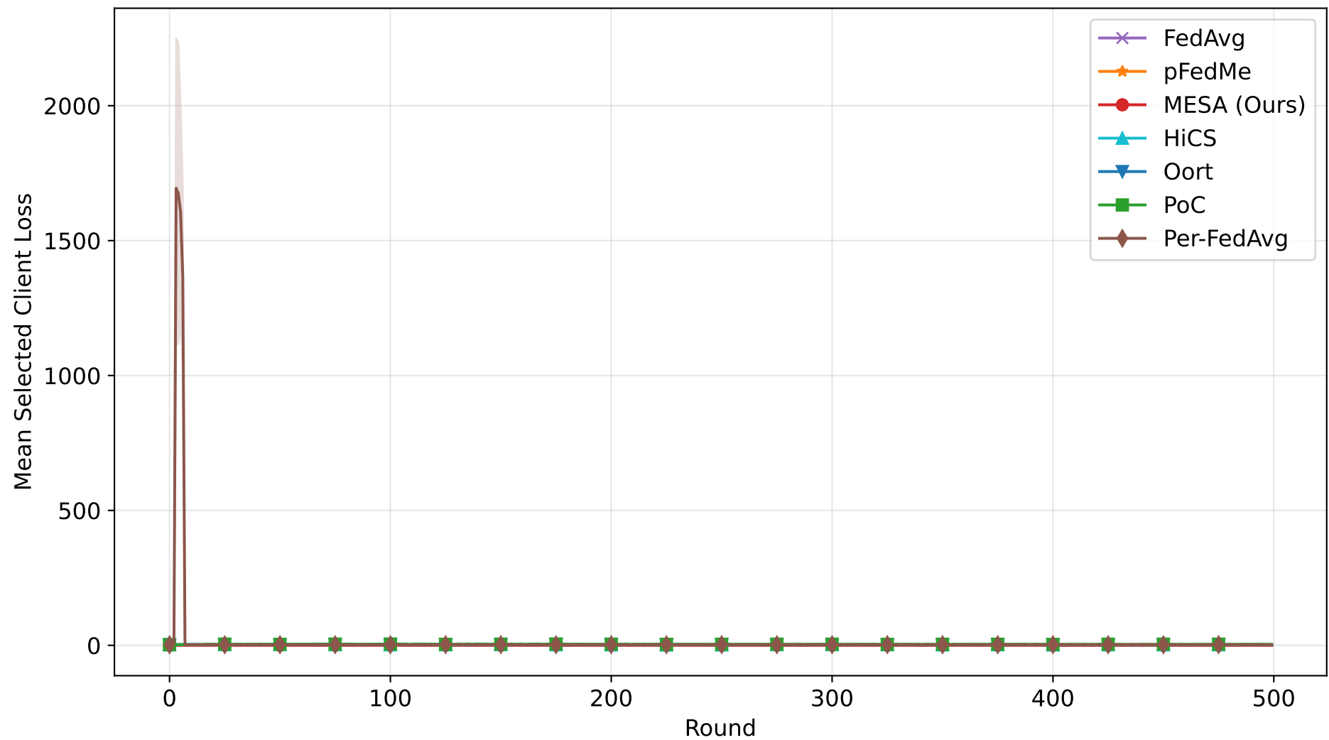
Cifar10 - CNN - Selected Client Loss Over Rounds
