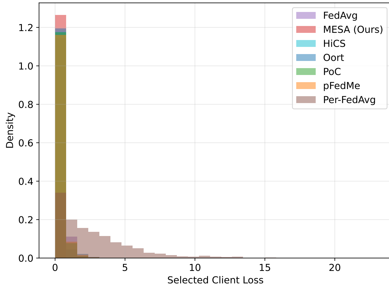
Distribution of Selected Client Losses
