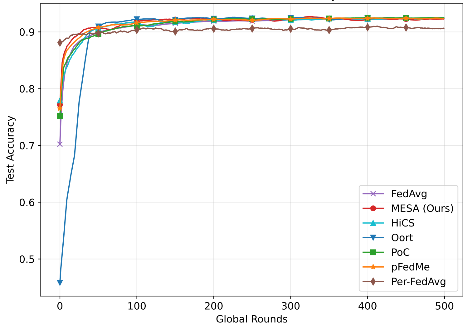
Mnist - MCLR - Test Accuracy
