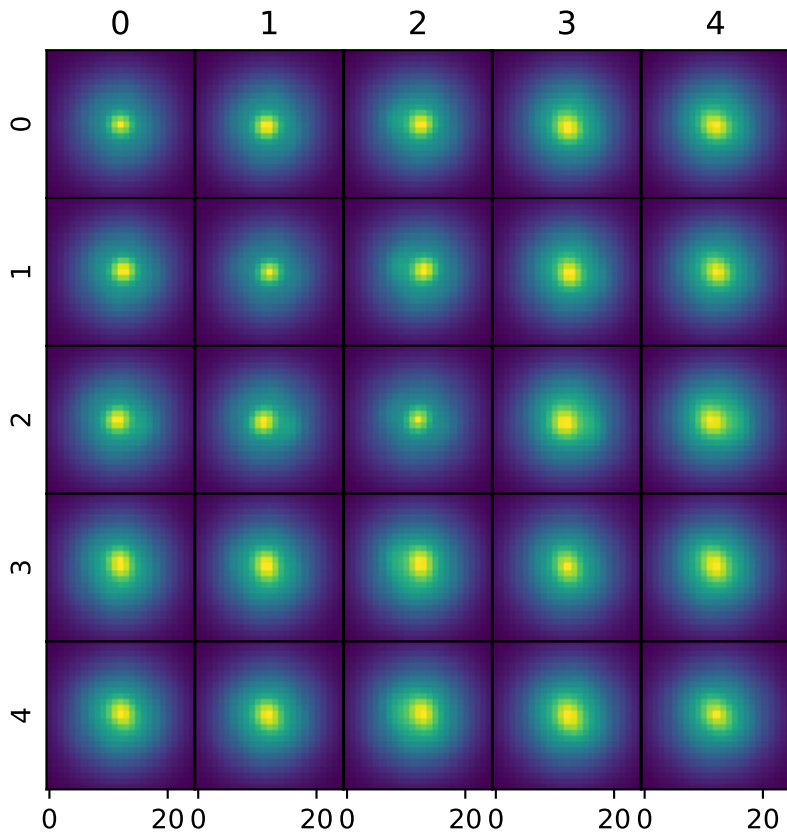
Cross-correlation of singular vectors
